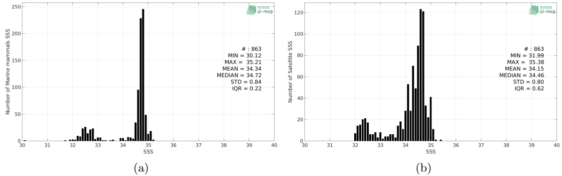
Figure 2: Histograms of SSS from Marine mammals (a) and SMOS SSS L3 v7 - 18 Days (CATDS-CECOS-LOCEAN) (b) considering all match-up pairs per bins of 0.1 over the North Atlantic Ocean Pi-MEP region and for the full satellite product period.
