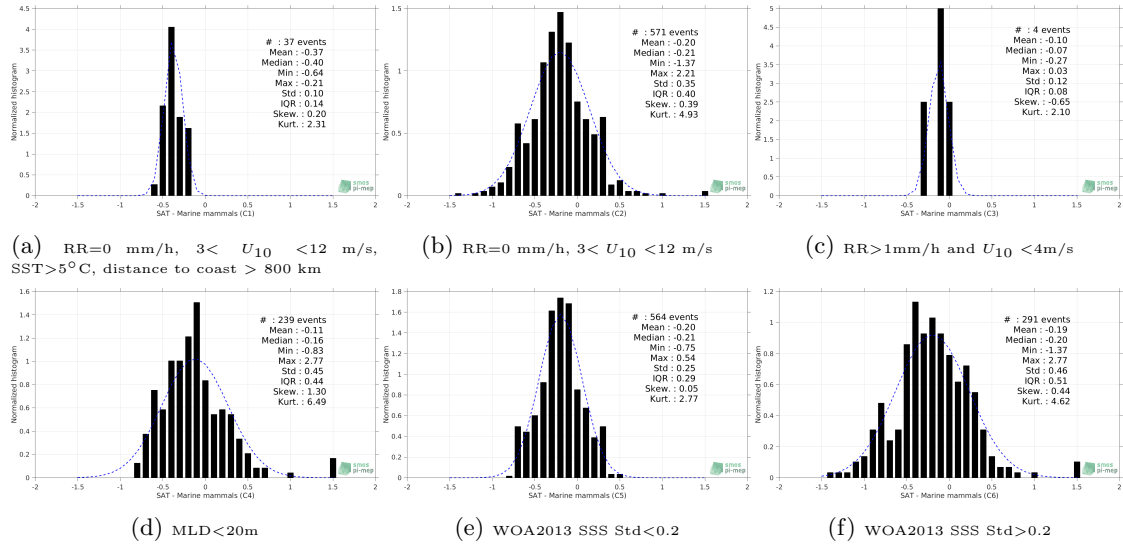
Figure 13: Normalized histogram of \Delta SSS (SMOS SSS L3 v7 - 18 Days (CATDS-CECOS-LOCEAN) - Marine mammals) for 6 different subdatasets corresponding to: RR=0 mm/h, 3 < U_{10} < 12 m/s, SST>5°C, distance to coast > 800 km (a), RR=0 mm/h, 3 < U_{10} < 12 m/s (b), RR>1mm/h and U_{10} < 4 m/s (c), MLD<20m (d), WOA2013 SSS Std<0.2 (e), WOA2013 SSS Std>0.2 (f).
