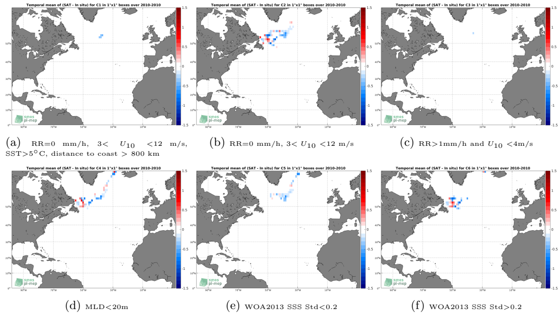
Figure 12: Temporal mean gridded over spatial boxes of size 1^{\circ}\times 1^{\circ} of \Delta\text{SSS} (SMOS SSS L3 v7 - 18 Days (CATDS-CECOS-LOCEAN) - Marine mammals) for 6 different subdatasets corresponding to:RR=0 mm/h, 3 < U_{10} < 12 m/s, SST >5^{\circ}\text{C} , distance to coast > 800 km (a), RR=0 mm/h, 3 < U_{10} < 12 m/s (b), RR >1\text{mm/h} and U_{10} < 4\text{m/s} (c),MLD <20\text{m} (d),WOA2013 SSS Std <0.2 (e),WOA2013 SSS Std >0.2 (f).
