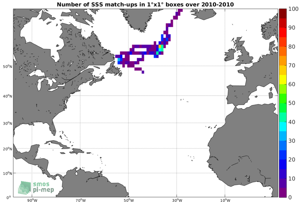
Figure 4: Number of SSS match-ups between Marine mammals SSS and the SMOS SSS L3 v7 - 18 Days (CATDS-CECOS-LOCEAN) SSS product for the North Atlantic Ocean Pi-MEP region over 1^{\circ} \times 1^{\circ} boxes and for the full satellite product period.
