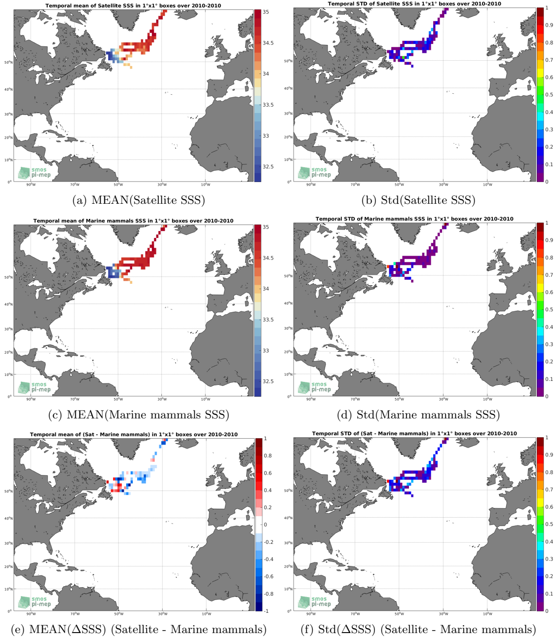
Figure 6: Temporal mean (left) and Std (right) of SSS from SMOS SSS L3 v7 - 18 Days (CATDS-CECOS-LOCEAN) (top), Marine mammals (middle), and of \Delta SSS (Satellite - Marine mammals). Only match-up pairs are used to generate these maps.
