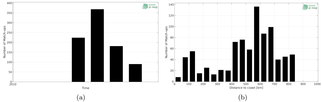
Figure 1: Number of match-ups between Marine mammals and SMOS SSS L3 v7 - 18 Days (CATDS-CECOS-LOCEAN) SSS as a function of time (a) and as function of the distance to coast (b) over the North Atlantic Ocean Pi-MEP region and for the full satellite product period.
