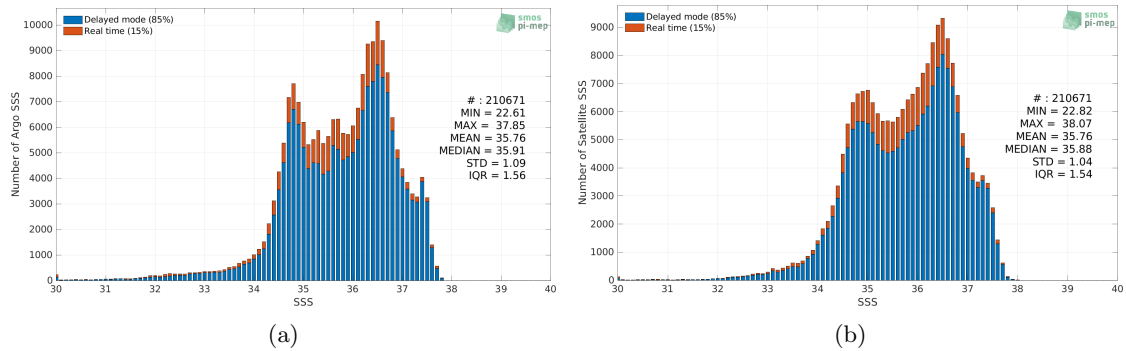
Figure 2: Histograms of SSS from Argo (a) and SMOS SSS L3 v7 - 18 Days (CATDS-CECOS-LOCEAN) (b) considering all match-up pairs per bins of 0.1 over the North Atlantic Ocean Pi-MEP region and for the full satellite product period.
