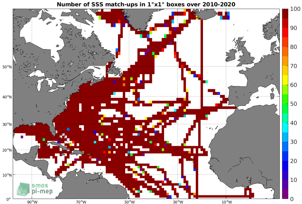
Figure 4: Number of SSS match-ups between TSG (SAMOS) SSS and the SMOS SSS L3 v5 - 9 Days (CATDS-CECOS-LOCEAN) SSS product for the North Atlantic Ocean Pi-MEP region over 1°x1° boxes and for the full satellite product period.
