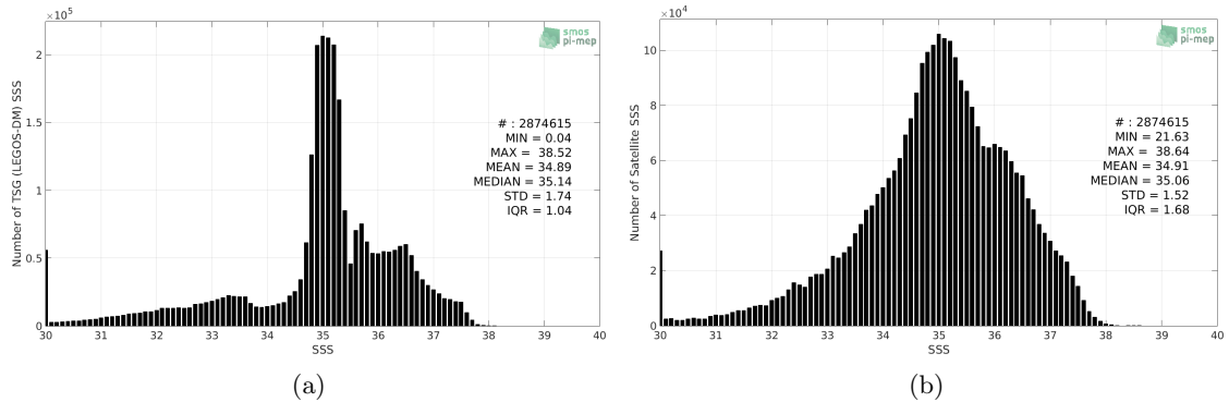
Figure 2: Histograms of SSS from TSG (LEGOS-DM) (a) and SMOS SSS L3 v5 - 9 Days (CATDS-CECOS-LOCEAN) (b) considering all match-up pairs per bins of 0.1 over the North Atlantic Ocean Pi-MEP region and for the full satellite product period.
