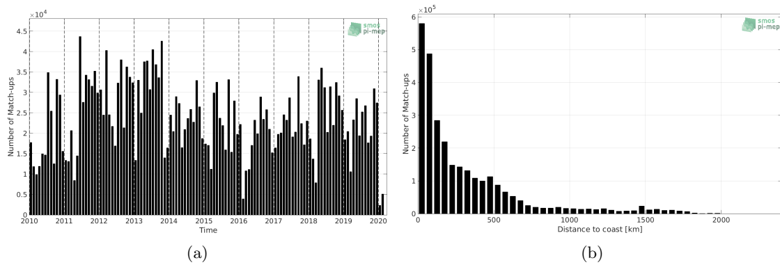
Figure 1: Number of match-ups between TSG (LEGOS-DM) and SMOS SSS L3 v5 - 9 Days (CATDS-CECOS-LOCEAN) SSS as a function of time (a) and as function of the distance to coast (b) over the North Atlantic Ocean Pi-MEP region and for the full satellite product period.
