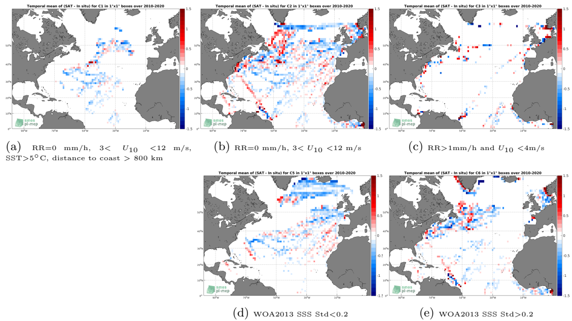
Figure 12: Temporal mean gridded over spatial boxes of size 1^\circ \times 1^\circ of \Delta\text{SSS} (SMOS SSS L3 v5 - 9 Days (CATDS-CECOS-LOCEAN) - TSG (LEGOS-DM)) for 5 different subdatasets corresponding to:RR=0 mm/h, 3 < U_{10} < 12 m/s, SST > 5^\circ\text{C} , distance to coast > 800 km (a), RR=0 mm/h, 3 < U_{10} < 12 m/s (b), RR > 1 mm/h and U_{10} < 4 m/s (c), WOA2013 SSS Std < 0.2 (d), WOA2013 SSS Std > 0.2 (e).
