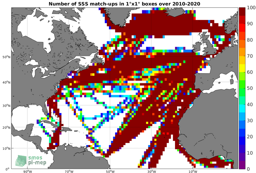
Figure 4: Number of SSS match-ups between TSG (LEGOS-DM) SSS and the SMOS SSS L3 v5 - 9 Days (CATDS-CECOS-LOCEAN) SSS product for the North Atlantic Ocean Pi-MEP region over 1^\circ \times 1^\circ boxes and for the full satellite product period.
