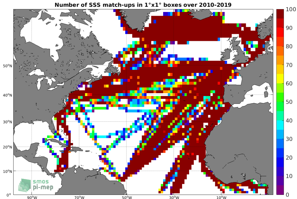
Figure 4: Number of SSS match-ups between TSG (LEGOS-DM) SSS and the SMOS SSS L3 v5 - 9 Days (CATDS-CECOS-LOCEAN) SSS product for the North Atlantic Ocean Pi-MEP region over 1°x1° boxes and for the full satellite product period.
