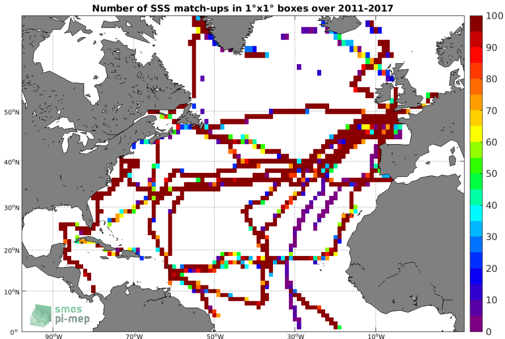
Figure 4: Number of SSS match-ups between TSG (GOSUD-Sailing-ship) SSS and the SMOS SSS L3 v5 - 9 Days (CATDS-CECOS-LOCEAN) SSS product for the North Atlantic Ocean Pi-MEP region over 1°x1° boxes and for the full satellite product period.
