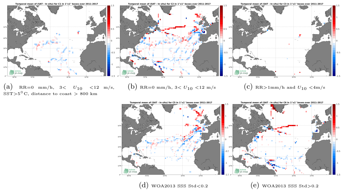
Figure 12: Temporal mean gridded over spatial boxes of size 1^\circ \times 1^\circ of \Delta\text{SSS} (SMOS SSS L3 v5 - 9 Days (CATDS-CECOS-LOCEAN) - TSG (GOSUD-Sailing-ship)) for 5 different subdatasets corresponding to: RR=0 mm/h, 3 < U_{10} < 12 m/s, SST > 5°C, distance to coast > 800 km (a), RR=0 mm/h, 3 < U_{10} < 12 m/s (b), RR > 1mm/h and U_{10} < 4 m/s (c), WOA2013 SSS Std < 0.2 (d), WOA2013 SSS Std > 0.2 (e).
