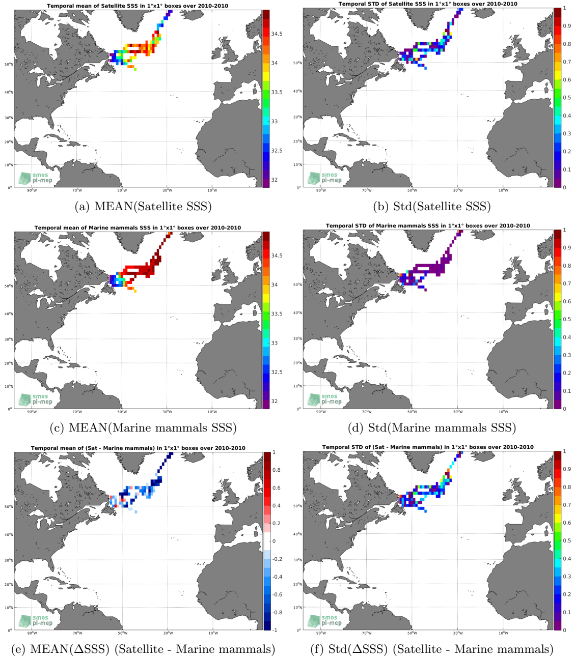
Figure 6: Temporal mean (left) and Std (right) of SSS from SMOS SSS L3 v5 - 9 Days (CATDS-CECOS-LOCEAN) (top), Marine mammals (middle), and of \Delta SSS (Satellite - Marine mammals). Only match-up pairs are used to generate these maps.
