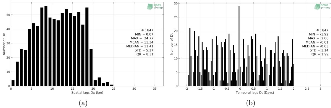
Figure 5: Histograms of the spatial (a) and temporal (b) lags between the location/time of the Marine mammals measurement and the date of the corresponding SMOS SSS L3 v5 - 9 Days (CATDS-CECOS-LOCEAN) SSS pixel.
