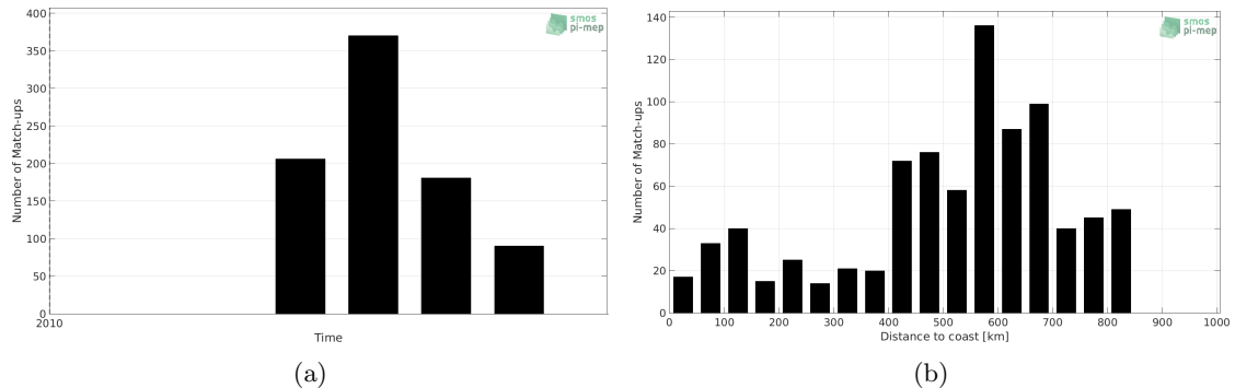
Figure 1: Number of match-ups between Marine mammals and SMOS SSS L3 v5 - 9 Days (CATDS-CECOS-LOCEAN) SSS as a function of time (a) and as function of the distance to coast (b) over the North Atlantic Ocean Pi-MEP region and for the full satellite product period.
