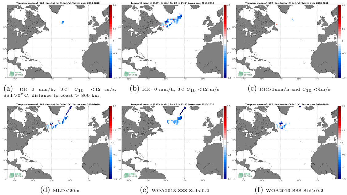
Figure 12: Temporal mean gridded over spatial boxes of size 1^{\circ}\times 1^{\circ} of \Delta\text{SSS} (SMOS SSS L3 v5 - 9 Days (CATDS-CECOS-LOCEAN) - Marine mammals) for 6 different subdatasets corresponding to:RR=0 mm/h, 3 < U_{10} < 12 m/s, SST >5^{\circ}\text{C} , distance to coast > 800 km (a), RR=0 mm/h, 3 < U_{10} < 12 m/s (b), RR >1\text{mm/h} and U_{10} < 4\text{m/s} (c),MLD <20\text{m} (d),WOA2013 SSS Std <0.2 (e),WOA2013 SSS Std >0.2 (f).
