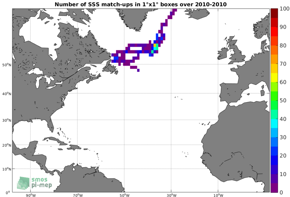
Figure 4: Number of SSS match-ups between Marine mammals SSS and the SMOS SSS L3 v5 - 9 Days (CATDS-CECOS-LOCEAN) SSS product for the North Atlantic Ocean Pi-MEP region over 1^\circ \times 1^\circ boxes and for the full satellite product period.
