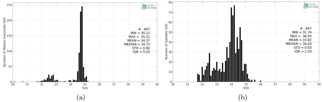
Figure 2: Histograms of SSS from Marine mammals (a) and SMOS SSS L3 v5 - 9 Days (CATDS-CECOS-LOCEAN) (b) considering all match-up pairs per bins of 0.1 over the North Atlantic Ocean Pi-MEP region and for the full satellite product period.
