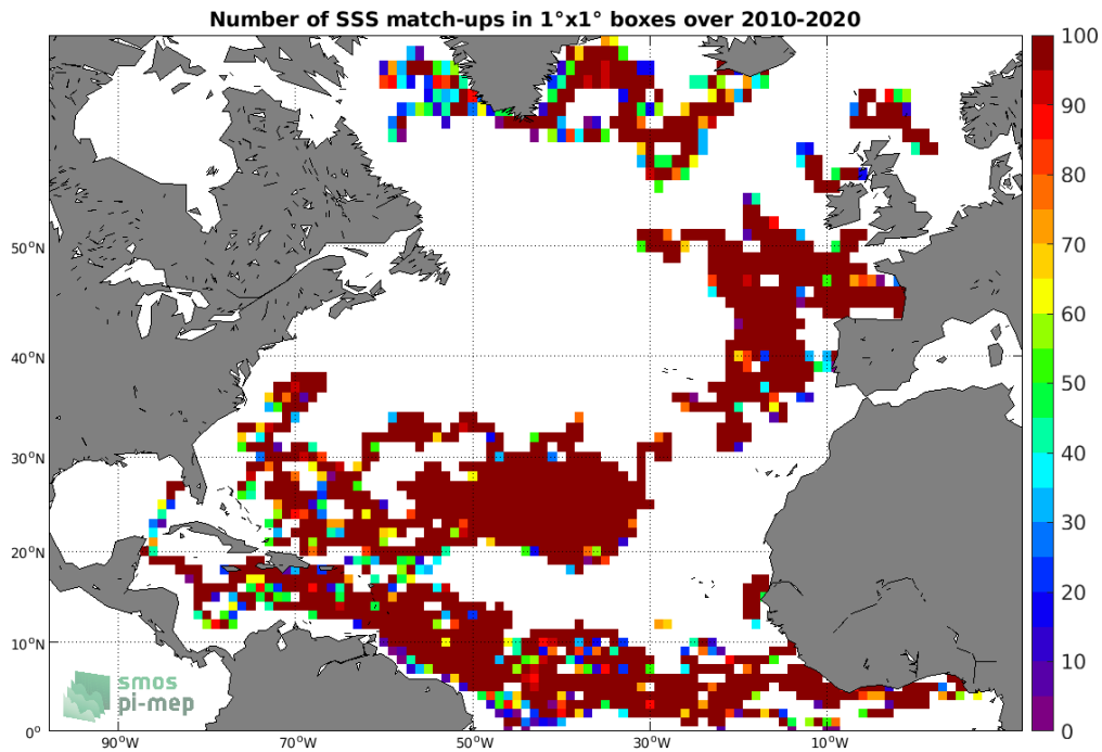
Figure 3: Number of SSS match-ups between Surface drifters SSS and the SMOS SSS L3 v5 - 9 Days (CATDS-CECOS-LOCEAN) SSS product for the North Atlantic Ocean Pi-MEP region over 1^\circ \times 1^\circ boxes and for the full satellite product period.
