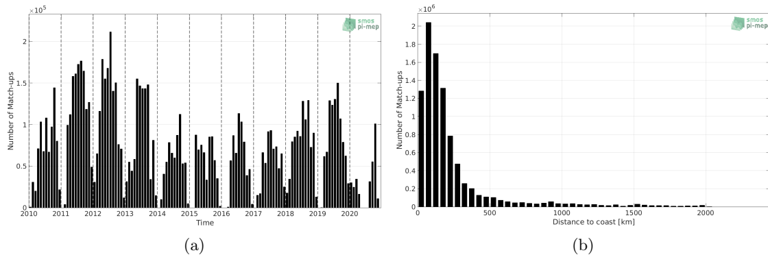
Figure 1: Number of match-ups between TSG (SAMOS) and SMOS SSS L3 v5 - 18 Days (CATDS-CECOS-LOCEAN) SSS as a function of time (a) and as function of the distance to coast (b) over the North Atlantic Ocean Pi-MEP region and for the full satellite product period.
