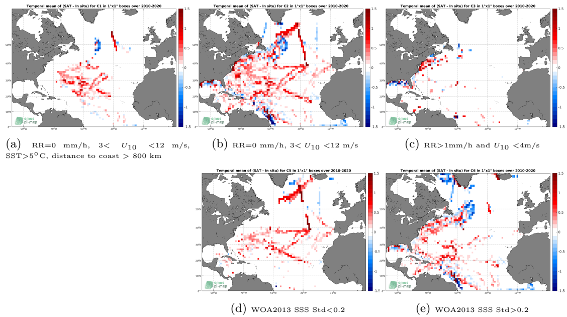
Figure 12: Temporal mean gridded over spatial boxes of size 1^\circ \times 1^\circ of \Delta\text{SSS} (SMOS SSS L3 v5 - 18 Days (CATDS-CECOS-LOCEAN) - TSG (SAMOS)) for 5 different subdatasets corresponding to:RR=0 mm/h, 3 < U_{10} < 12 m/s, SST >5^\circ\text{C} , distance to coast > 800 km (a), RR=0 mm/h, 3 < U_{10} < 12 m/s (b), RR >1 mm/h and U_{10} < 4 m/s (c), WOA2013 SSS Std <0.2 (d), WOA2013 SSS Std >0.2 (e).
