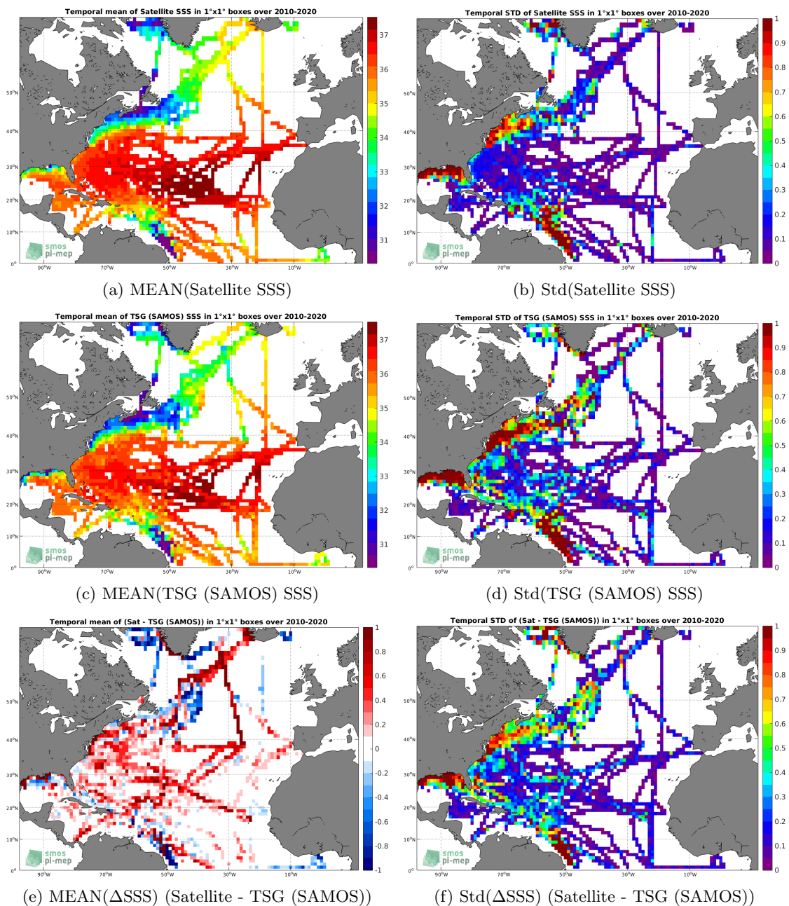
Figure 6: Temporal mean (left) and Std (right) of SSS from SMOS SSS L3 v5 - 18 Days (CATDS-CECOS-LOCEAN) (top), TSG (SAMOS) (middle), and of \Delta SSS (Satellite - TSG (SAMOS)). Only match-up pairs are used to generate these maps.
