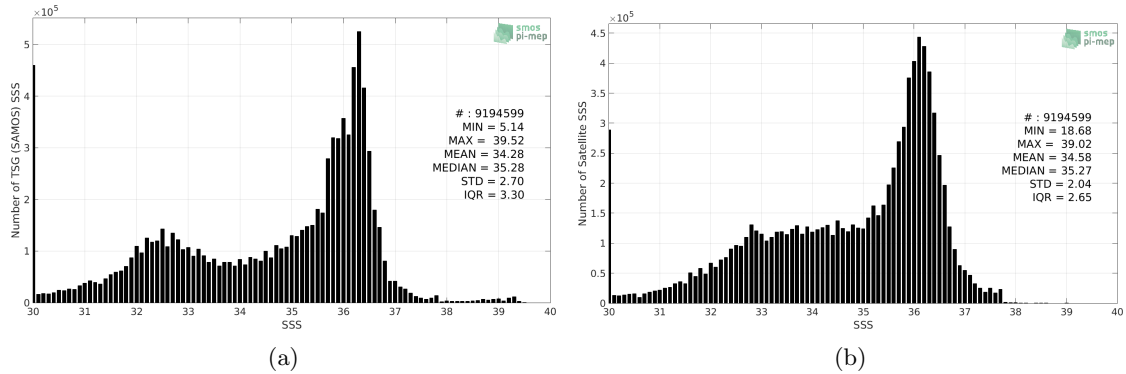
Figure 2: Histograms of SSS from TSG (SAMOS) (a) and SMOS SSS L3 v5 - 18 Days (CATDS-CECOS-LOCEAN) (b) considering all match-up pairs per bins of 0.1 over the North Atlantic Ocean Pi-MEP region and for the full satellite product period.
