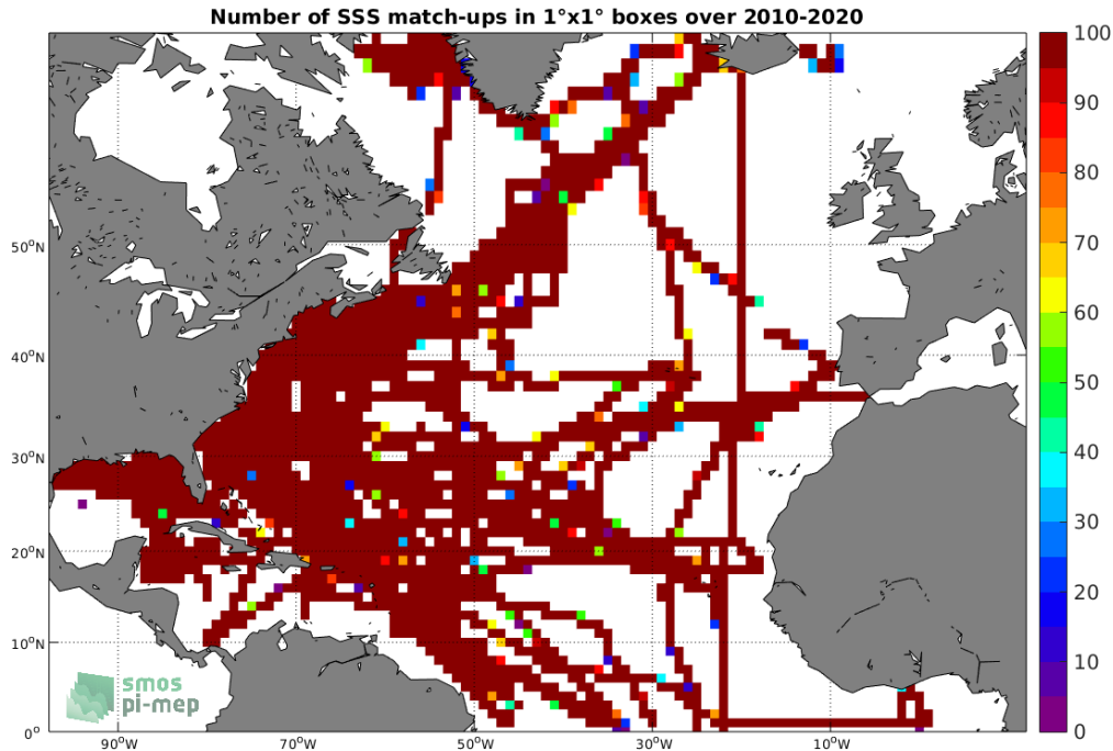
Figure 4: Number of SSS match-ups between TSG (SAMOS) SSS and the SMOS SSS L3 v5 - 18 Days (CATDS-CECOS-LOCEAN) SSS product for the North Atlantic Ocean Pi-MEP region over 1^\circ \times 1^\circ boxes and for the full satellite product period.
