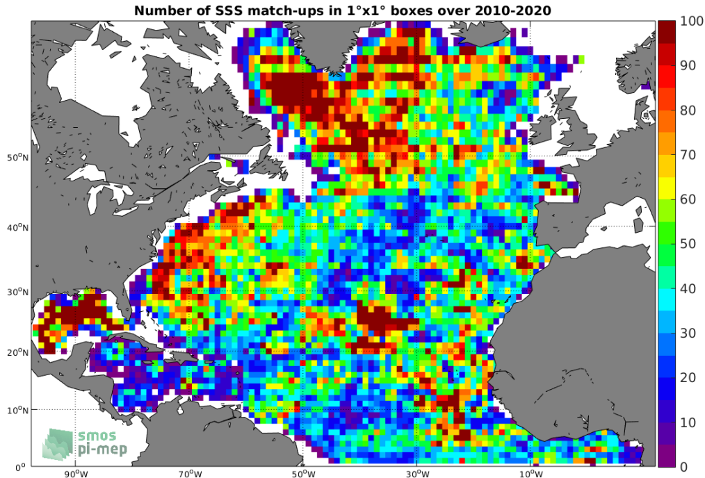
Figure 4: Number of SSS match-ups between Argo SSS and the SMOS SSS L3 v5 - 18 Days (CATDS-CECOS-LOCEAN) SSS product for the North Atlantic Ocean Pi-MEP region over 1^\circ \times 1^\circ boxes and for the full satellite product period.
