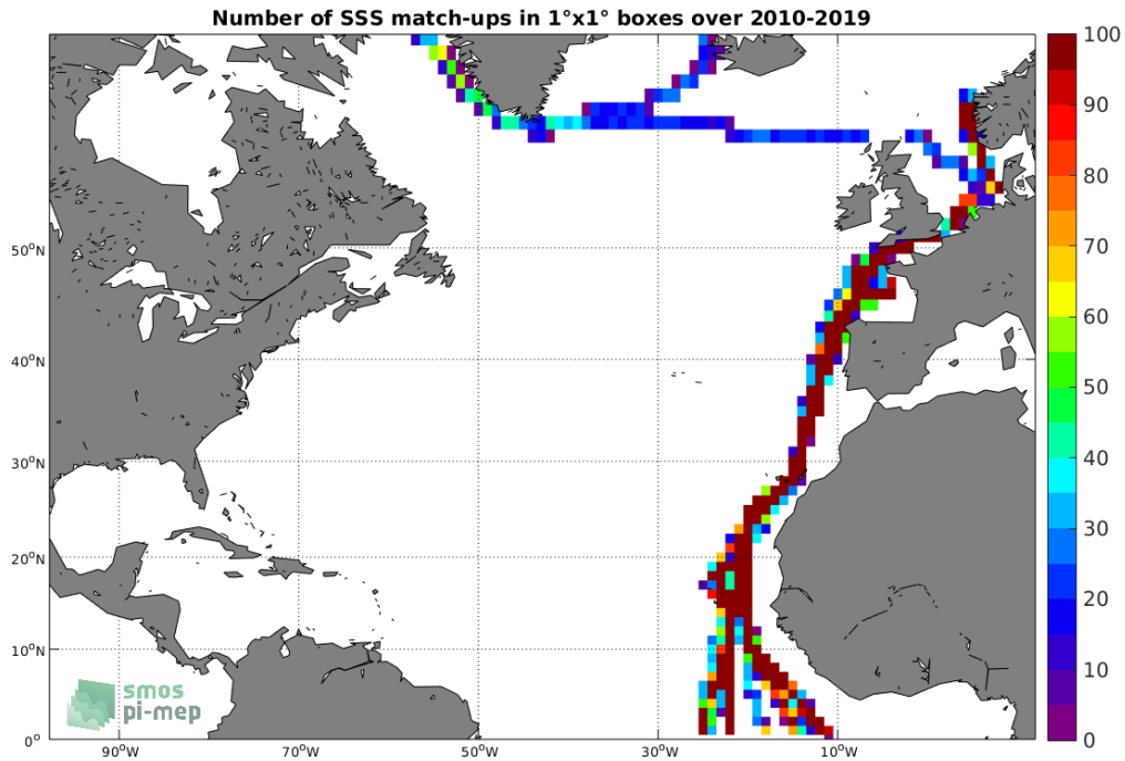
Figure 4: Number of SSS match-ups between TSG (Polarstern) SSS and the SMOS SSS L3 v4 - 9 Days (CATDS-CECOS-LOCEAN) SSS product for the North Atlantic Ocean Pi-MEP region over 1°x1° boxes and for the full satellite product period.
