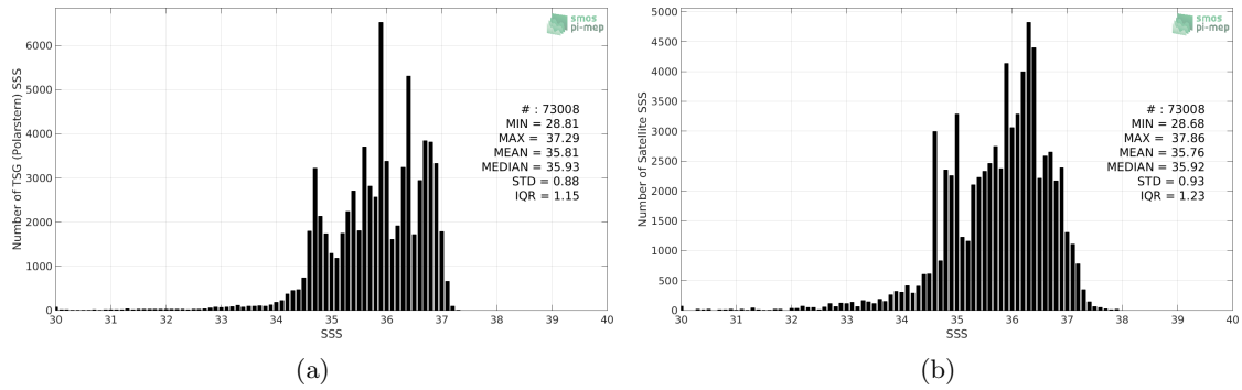
Figure 2: Histograms of SSS from TSG (Polarstern) (a) and SMOS SSS L3 v4 - 9 Days (CATDS-CECOS-LOCEAN) (b) considering all match-up pairs per bins of 0.1 over the North Atlantic Ocean Pi-MEP region and for the full satellite product period.
