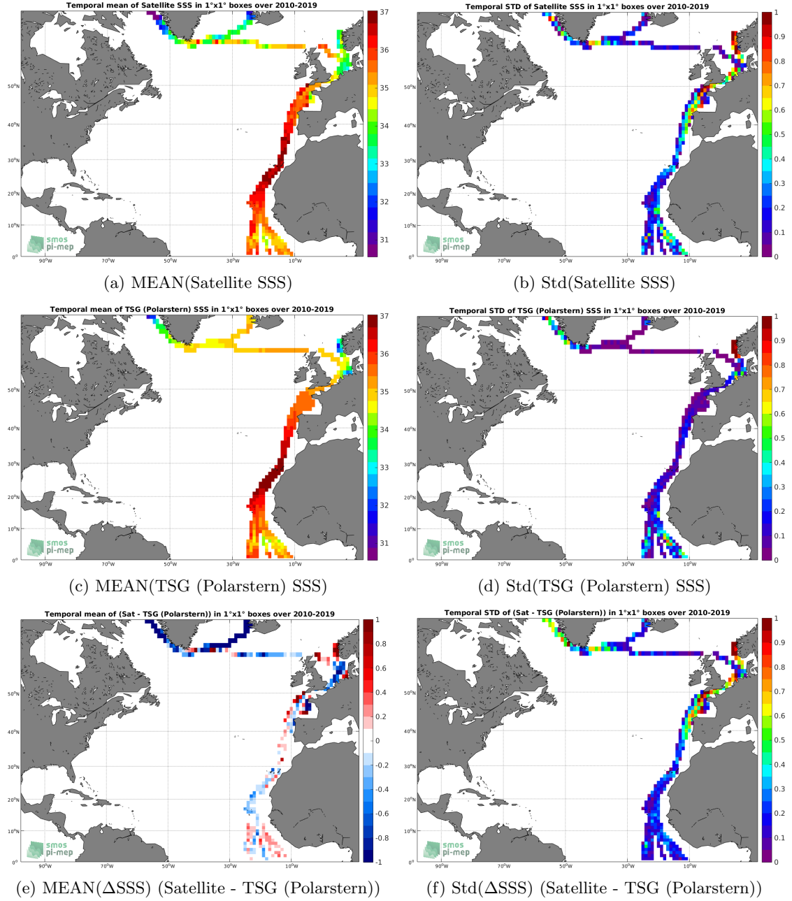
Figure 6: Temporal mean (left) and Std (right) of SSS from SMOS SSS L3 v4 - 9 Days (CATDS-CECOS-LOCEAN) (top), TSG (Polarstern) (middle), and of \Delta SSS (Satellite - TSG (Polarstern)). Only match-up pairs are used to generate these maps.
