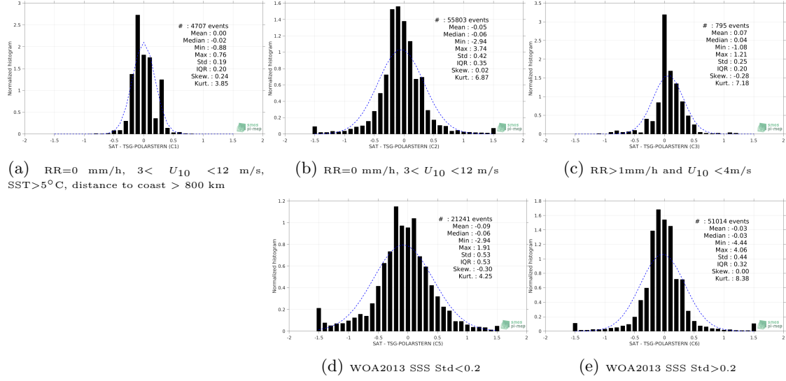
Figure 13: Normalized histogram of \Delta\text{SSS} (SMOS-L3-CATDS-CECOS-LOCEAN-V4-9DAYS-25KM - TSG-POLARSTERN) for 5 different subdatasets corresponding to: RR=0 mm/h, 3 < U_{10} < 12 m/s, SST > 5^\circ\text{C} , distance to coast > 800 km (a), RR=0 mm/h, 3 < U_{10} < 12 m/s (b), RR > 1\text{mm/h} and U_{10} < 4\text{m/s} (c), WOA2013 SSS Std < 0.2 (d), WOA2013 SSS Std > 0.2 (e).
