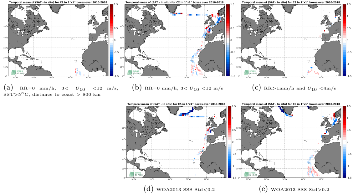
Figure 12: Temporal mean gridded over spatial boxes of size 1^\circ \times 1^\circ of \Delta SSS (SMOS-L3-CATDS-CECOS-LOCEAN-V4-9DAYS-25KM - TSG-POLARSTERN) for 5 different subdatasets corresponding to: RR=0 mm/h, 3 < U_{10} < 12 m/s, SST >5^\circ\text{C} , distance to coast > 800 km (a), RR=0 mm/h, 3 < U_{10} < 12 m/s (b), RR >1 mm/h and U_{10} < 4 m/s (c), WOA2013 SSS Std <0.2 (d), WOA2013 SSS Std >0.2 (e).
