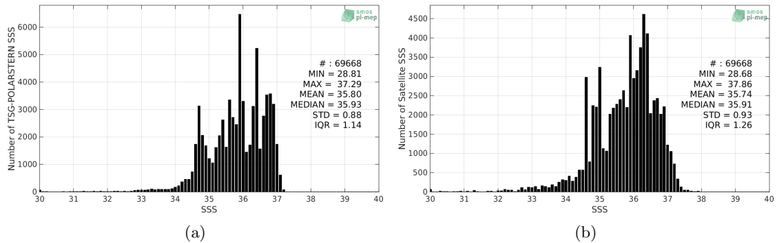
Figure 2: Histograms of SSS from TSG-POLARSTERN (a) and SMOS-L3-CATDS-CECOS-LOCEAN-V4-9DAYS-25KM (b) considering all match-up pairs per bins of 0.1 over the North Atlantic Ocean Pi-MEP region and for the full satellite product period.
