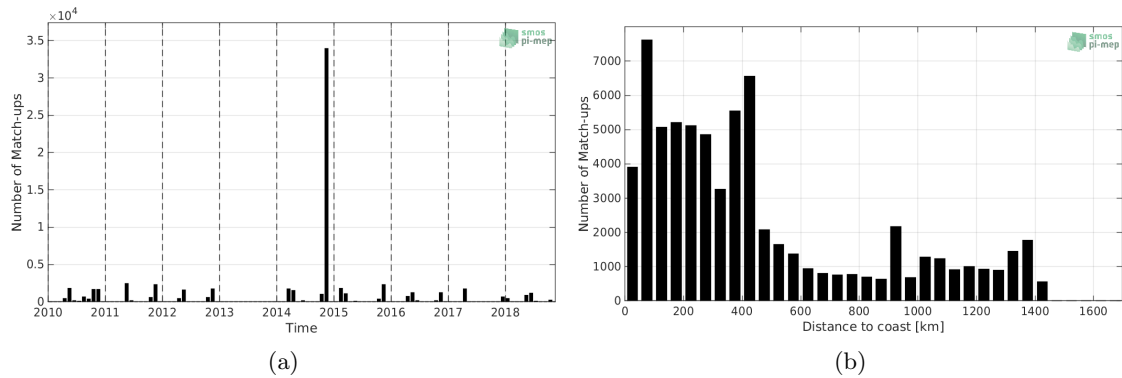
Figure 1: Number of match-ups between TSG-POLARSTERN and SMOS-L3-CATDS-CECOS-LOCEAN-V4-9DAYS-25KM SSS as a function of time (a) and as function of the distance to coast (b) over the North Atlantic Ocean Pi-MEP region and for the full satellite product period.
