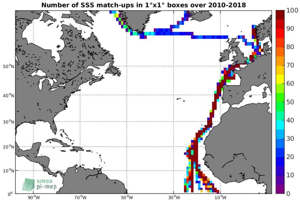
Figure 4: Number of SSS match-ups between TSG-POLARSTERN SSS and the SMOS-L3-CATDS-CECOS-LOCEAN-V4-9DAYS-25KM SSS product for the North Atlantic Ocean Pi-MEP region over 1^\circ \times 1^\circ boxes and for the full satellite product period.
