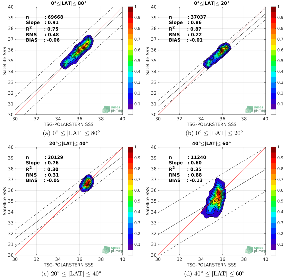
Figure 9: Contour maps of the concentration of SMOS-L3-CATDS-CECOS-LOCEAN-V4-9DAYS-25KM SSS (y-axis) versus TSG-POLARSTERN SSS (x-axis) at match-up pairs for different latitude bands. For each plot, the red line shows x=y . The black thin and dashed lines indicate a linear fit through the data cloud and the \pm 95\% confidence levels, respectively. The number match-up pairs n , the slope and R^2 coefficient of the linear fit, the root mean square (RMS) and the mean bias between satellite and in situ data are indicated for each latitude band in each plots.
