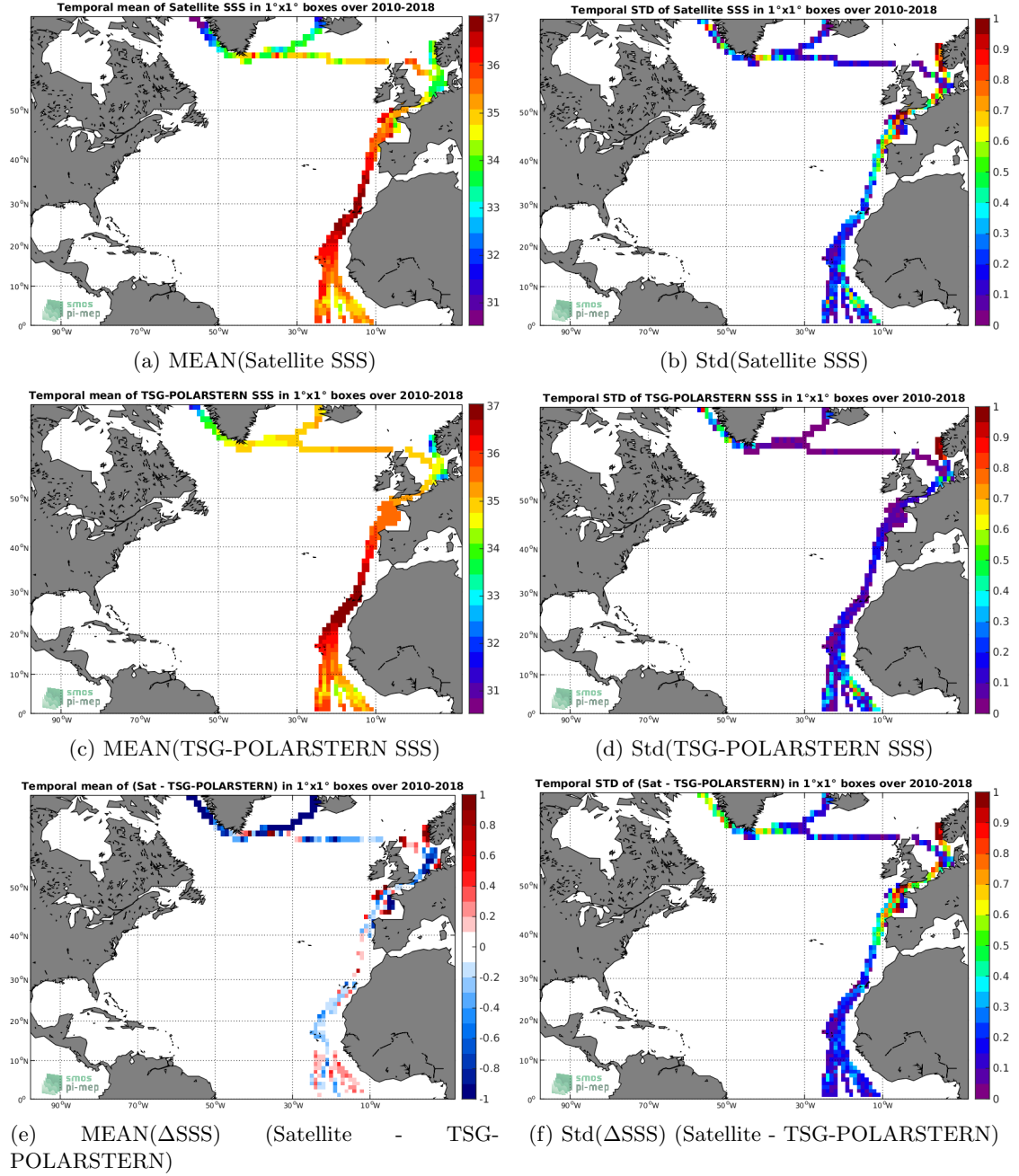
Figure 6: Temporal mean (left) and Std (right) of SSS from SMOS-L3-CATDS-CECOS-LOCEAN-V4-9DAYS-25KM (top), TSG-POLARSTERN (middle), and of \Delta SSS (Satellite - TSG-POLARSTERN). Only match-up pairs are used to generate these maps.
