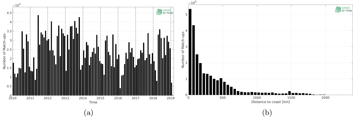
Figure 1: Number of match-ups between TSG-LEGOS-DM and SMOS-L3-CATDS-CECOS-LOCEAN-V4-9DAYS-25KM SSS as a function of time (a) and as function of the distance to coast (b) over the North Atlantic Ocean Pi-MEP region and for the full satellite product period.
