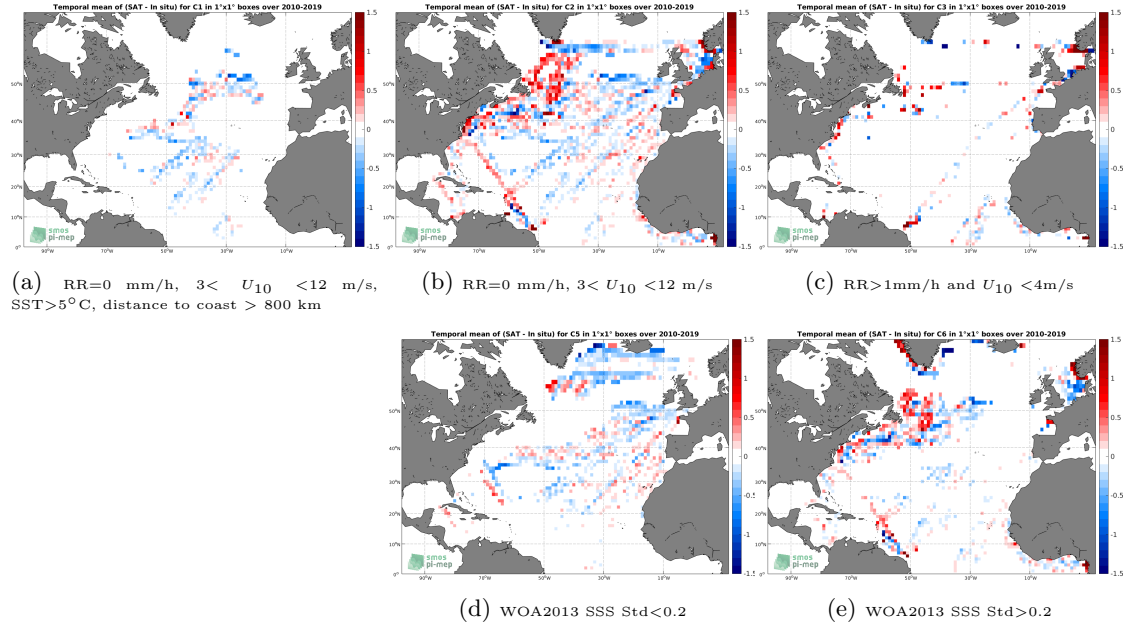
Figure 12: Temporal mean gridded over spatial boxes of size 1^\circ \times 1^\circ of \Delta SSS (SMOS-L3-CATDS-CECOS-LOCEAN-V4-9DAYS-25KM - TSG-LEGOS-DM) for 5 different subdatasets corresponding to: RR=0 mm/h, 3 < U_{10} < 12 m/s, SST > 5^\circ C , distance to coast > 800 km (a), RR=0 mm/h, 3 < U_{10} < 12 m/s (b), RR > 1 mm/h and U_{10} < 4 m/s (c), WOA2013 SSS Std < 0.2 (d), WOA2013 SSS Std > 0.2 (e).
