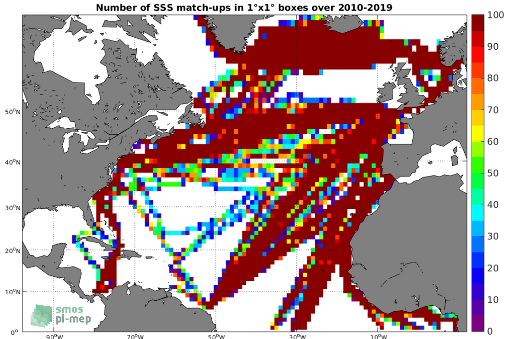
Figure 4: Number of SSS match-ups between TSG-LEGOS-DM SSS and the SMOS-L3-CATDS-CECOS-LOCEAN-V4-9DAYS-25KM SSS product for the North Atlantic Ocean Pi-MEP region over 1^\circ \times 1^\circ boxes and for the full satellite product period.
