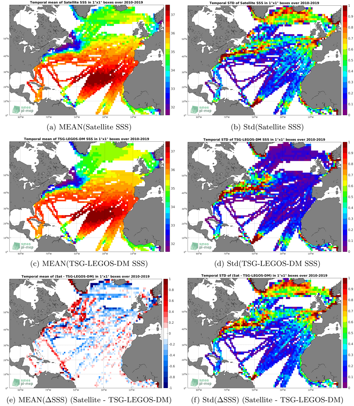
Figure 6: Temporal mean (left) and Std (right) of SSS from SMOS-L3-CATDS-CECOS-LOCEAN-V4-9DAYS-25KM (top), TSG-LEGOS-DM (middle), and of \Delta SSS (Satellite - TSG-LEGOS-DM). Only match-up pairs are used to generate these maps.
