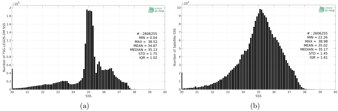
Figure 2: Histograms of SSS from TSG-LEGOS-DM (a) and SMOS-L3-CATDS-CECOS-LOCEAN-V4-9DAYS-25KM (b) considering all match-up pairs per bins of 0.1 over the North Atlantic Ocean Pi-MEP region and for the full satellite product period.
