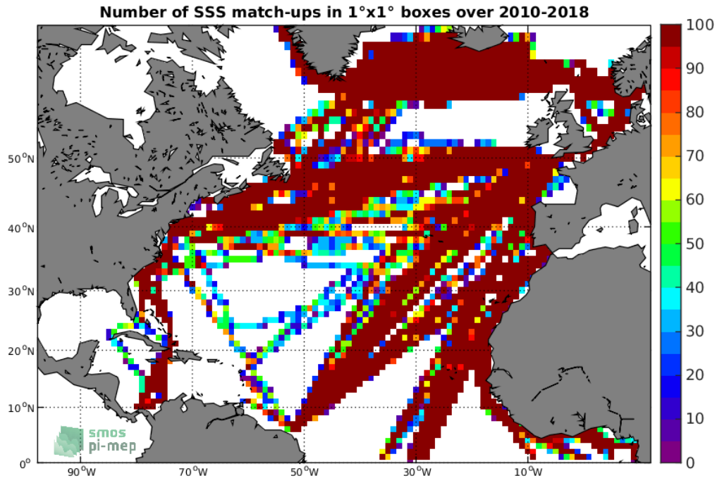
Figure 4: Number of SSS match-ups between TSG-LEGOS-DM SSS and the SMOS-L3-CATDS-CECOS-LOCEAN-V4-9DAYS-25KM SSS product for the North Atlantic Ocean Pi-MEP region over 1°x1° boxes and for the full satellite product period.
