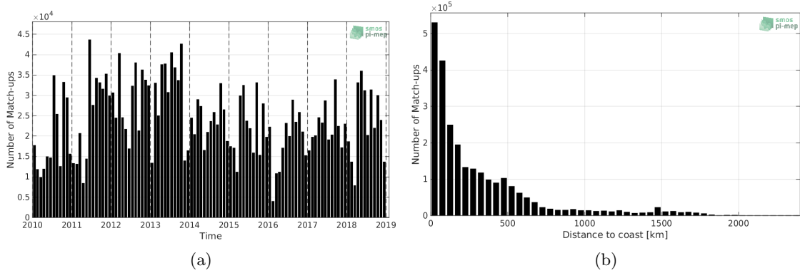
Figure 1: Number of match-ups between TSG-LEGOS-DM and SMOS-L3-CATDS-CECOS-LOCEAN-V4-9DAYS-25KM SSS as a function of time (a) and as function of the distance to coast (b) over the North Atlantic Ocean Pi-MEP region and for the full satellite product period.
