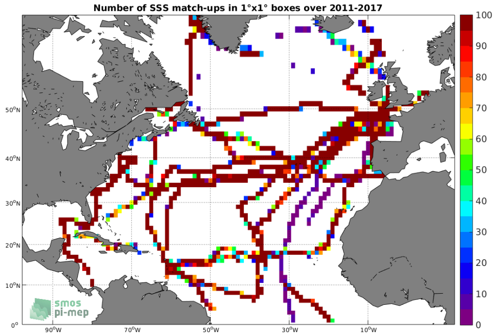
Figure 4: Number of SSS match-ups between TSG (GOSUD-Sailing-ship) SSS and the SMOS SSS L3 v4 - 9 Days (CATDS-CECOS-LOCEAN) SSS product for the North Atlantic Ocean Pi-MEP region over 1^\circ \times 1^\circ boxes and for the full satellite product period.
