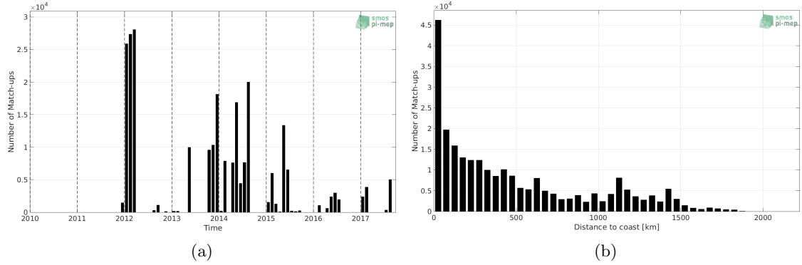
Figure 1: Number of match-ups between TSG (GOSUD-Sailing-ship) and SMOS SSS L3 v4 - 9 Days (CATDS-CECOS-LOCEAN) SSS as a function of time (a) and as function of the distance to coast (b) over the North Atlantic Ocean Pi-MEP region and for the full satellite product period.
