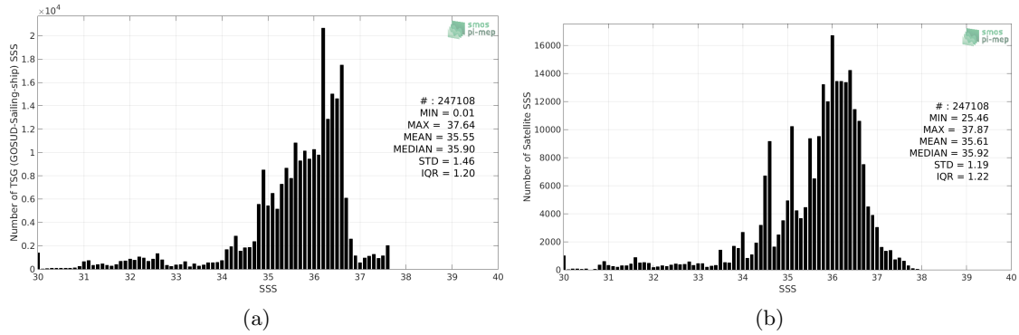
Figure 2: Histograms of SSS from TSG (GOSUD-Sailing-ship) (a) and SMOS SSS L3 v4 - 9 Days (CATDS-CECOS-LOCEAN) (b) considering all match-up pairs per bins of 0.1 over the North Atlantic Ocean Pi-MEP region and for the full satellite product period.
