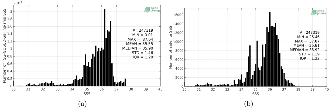
Figure 2: Histograms of SSS from TSG-GOSUD-Sailing-ship (a) and SMOS-L3-CATDS-CECOS-LOCEAN-V4-9DAYS-25KM (b) considering all match-up pairs per bins of 0.1 over the North Atlantic Ocean Pi-MEP region and for the full satellite product period.
