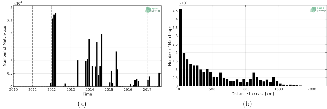
Figure 1: Number of match-ups between TSG-GOSUD-Sailing-ship and SMOS-L3-CATDS-CECOS-LOCEAN-V4-9DAYS-25KM SSS as a function of time (a) and as function of the distance to coast (b) over the North Atlantic Ocean Pi-MEP region and for the full satellite product period.
