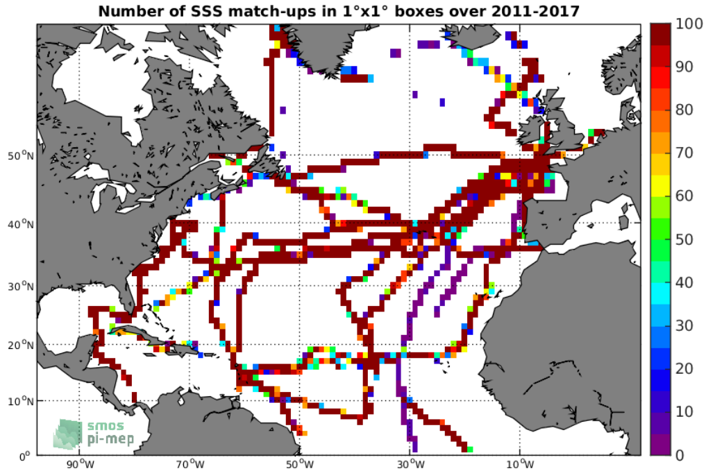
Figure 4: Number of SSS match-ups between TSG-GOSUD-Sailing-ship SSS and the SMOS-L3-CATDS-CECOS-LOCEAN-V4-9DAYS-25KM SSS product for the North Atlantic Ocean Pi-MEP region over 1°x1° boxes and for the full satellite product period.
