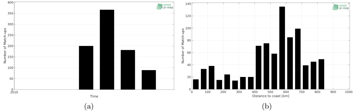
Figure 1: Number of match-ups between Sea mammals and SMOS SSS L3 v4 - 9 Days (CATDS-CECOS-LOCEAN) SSS as a function of time (a) and as function of the distance to coast (b) over the North Atlantic Ocean Pi-MEP region and for the full satellite product period.
