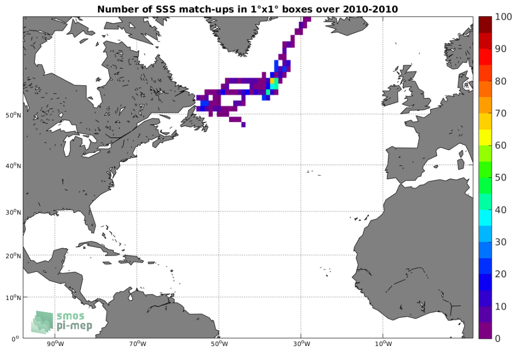
Figure 4: Number of SSS match-ups between Sea mammals SSS and the SMOS SSS L3 v4 - 9 Days (CATDS-CECOS-LOCEAN) SSS product for the North Atlantic Ocean Pi-MEP region over 1°x1° boxes and for the full satellite product period.
