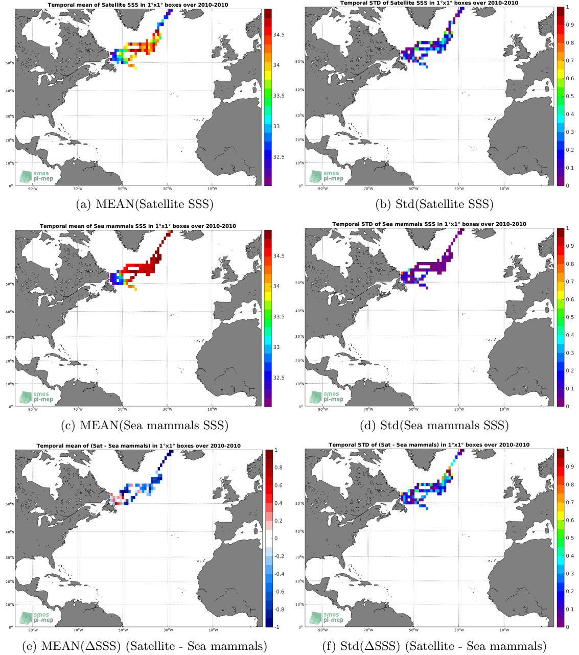
Figure 6: Temporal mean (left) and Std (right) of SSS from SMOS SSS L3 v4 - 9 Days (CATDS-CECOS-LOCEAN) (top), Sea mammals (middle), and of \Delta SSS (Satellite - Sea mammals). Only match-up pairs are used to generate these maps.
