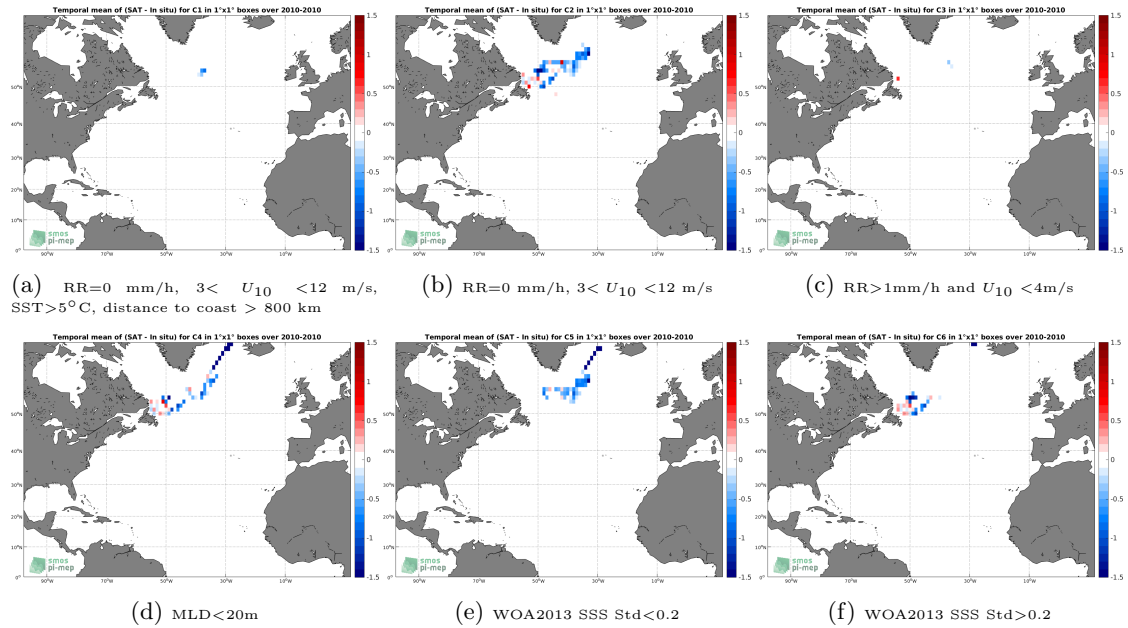
Figure 12: Temporal mean gridded over spatial boxes of size 1^{\circ}\times 1^{\circ} of \Delta\text{SSS} (SMOS SSS L3 v4 - 9 Days (CATDS-CECOS-LOCEAN) - Sea mammals) for 6 different subdatasets corresponding to:RR=0 mm/h, 3 < U_{10} < 12 m/s, SST >5^{\circ}\text{C} , distance to coast > 800 km (a), RR=0 mm/h, 3 < U_{10} < 12 m/s (b), RR >1\text{mm/h} and U_{10} < 4\text{m/s} (c),MLD <20\text{m} (d),WOA2013 SSS Std <0.2 (e),WOA2013 SSS Std >0.2 (f).
