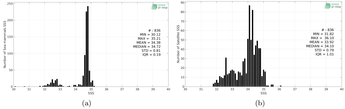
Figure 2: Histograms of SSS from Sea mammals (a) and SMOS SSS L3 v4 - 9 Days (CATDS-CECOS-LOCEAN) (b) considering all match-up pairs per bins of 0.1 over the North Atlantic Ocean Pi-MEP region and for the full satellite product period.
