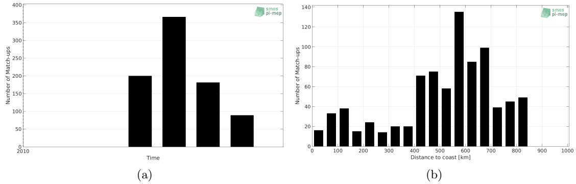
Figure 1: Number of match-ups between Sea mammals and SMOS-L3-CATDS-CECOS-LOCEAN-V4-9DAYS-25KM SSS as a function of time (a) and as function of the distance to coast (b) over the North Atlantic Ocean Pi-MEP region and for the full satellite product period.
