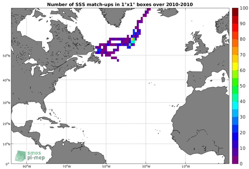
Figure 4: Number of SSS match-ups between Sea mammals SSS and the SMOS-L3-CATDS-CECOS-LOCEAN-V4-9DAYS-25KM SSS product for the North Atlantic Ocean Pi-MEP region over 1^\circ \times 1^\circ boxes and for the full satellite product period.
