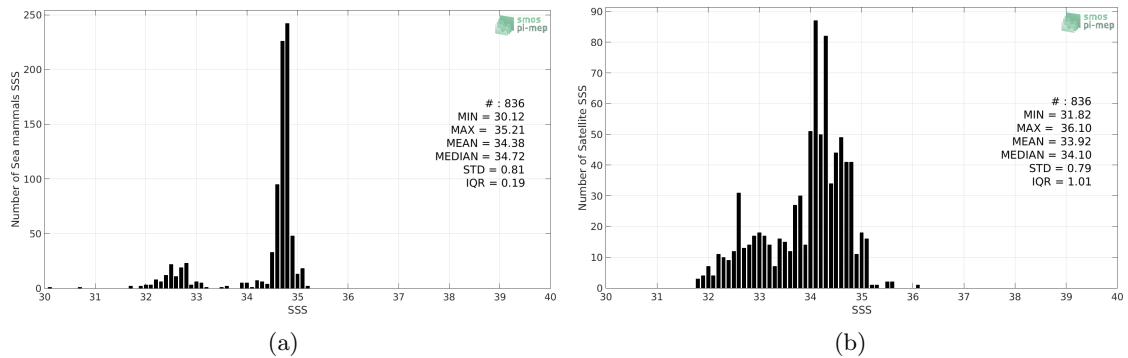
Figure 2: Histograms of SSS from Sea mammals (a) and SMOS-L3-CATDS-CECOS-LOCEAN-V4-9DAYS-25KM (b) considering all match-up pairs per bins of 0.1 over the North Atlantic Ocean Pi-MEP region and for the full satellite product period.
