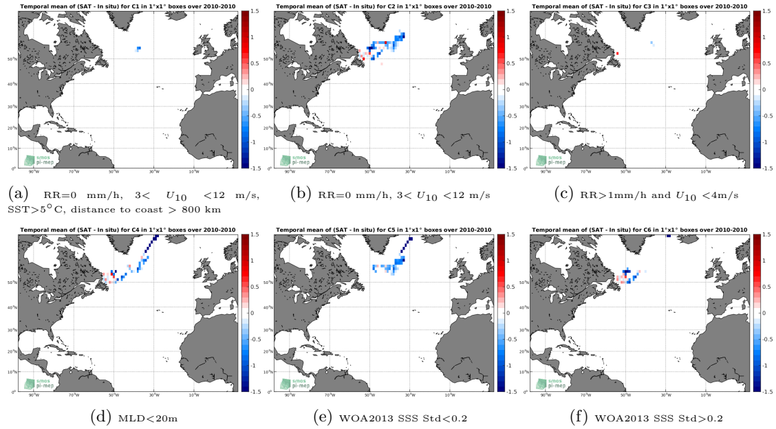
Figure 12: Temporal mean gridded over spatial boxes of size 1^\circ \times 1^\circ of \Delta SSS (SMOS-L3-CATDS-CECOS-LOCEAN-V4-9DAYS-25KM - Sea mammals) for 6 different subdatasets corresponding to: RR=0 mm/h, 3 < U_{10} < 12 m/s, SST > 5^\circ C , distance to coast > 800 km (a), RR=0 mm/h, 3 < U_{10} < 12 m/s (b), RR > 1 mm/h and U_{10} < 4 m/s (c), MLD < 20 m (d), WOA2013 SSS Std < 0.2 (e), WOA2013 SSS Std > 0.2 (f).
