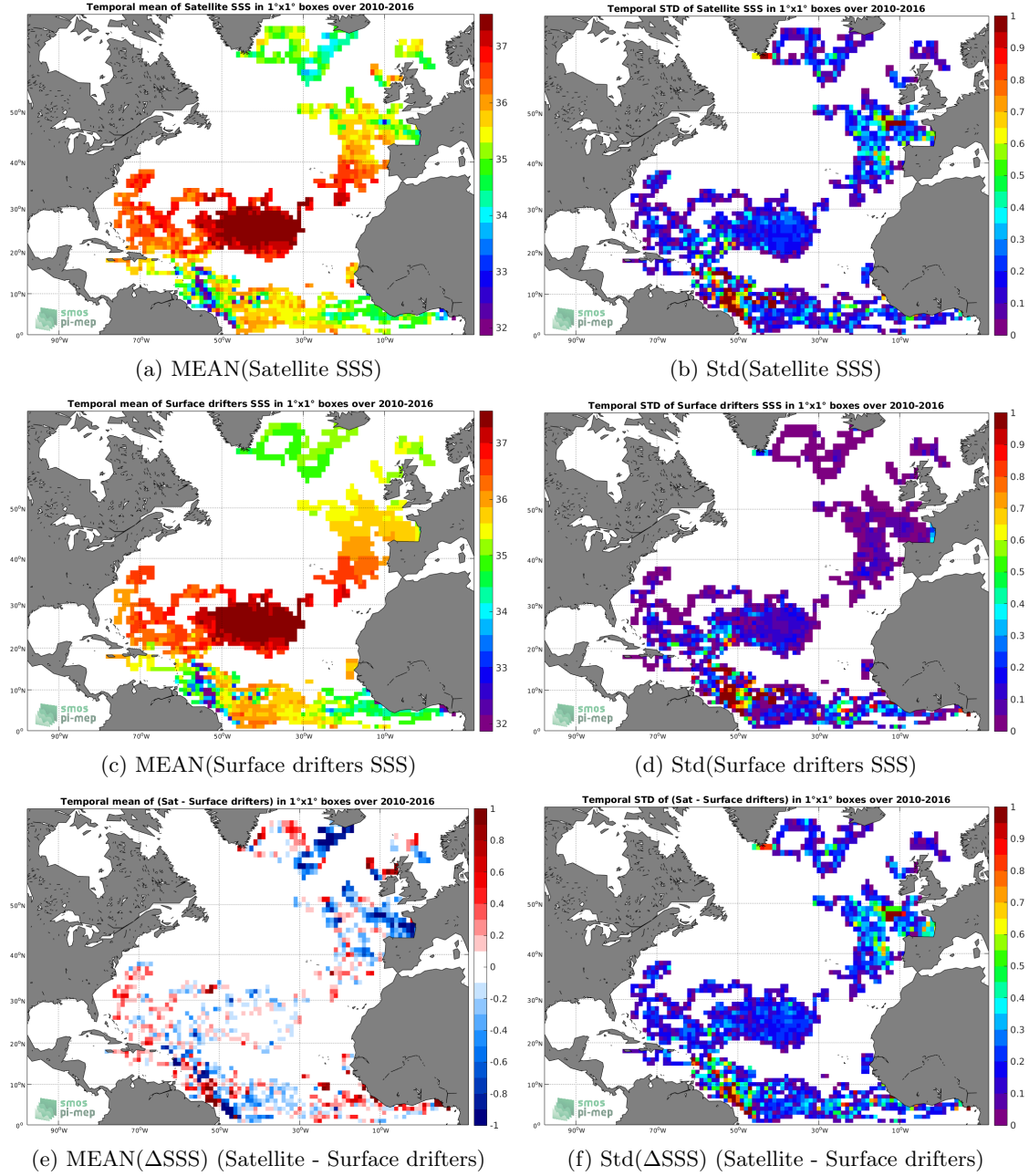
Figure 5: Temporal mean (left) and Std (right) of SSS from SMOS SSS L3 v4 - 9 Days (CATDS-CECOS-LOCEAN) (top), Surface drifters (middle), and of \Delta SSS (Satellite - Surface drifters). Only match-up pairs are used to generate these maps.
