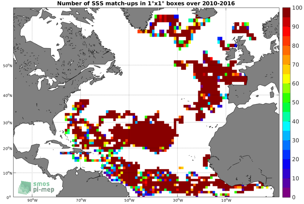
Figure 3: Number of SSS match-ups between Surface drifters SSS and the SMOS SSS L3 v4 - 9 Days (CATDS-CECOS-LOCEAN) SSS product for the North Atlantic Ocean Pi-MEP region over 1°x1° boxes and for the full satellite product period.
