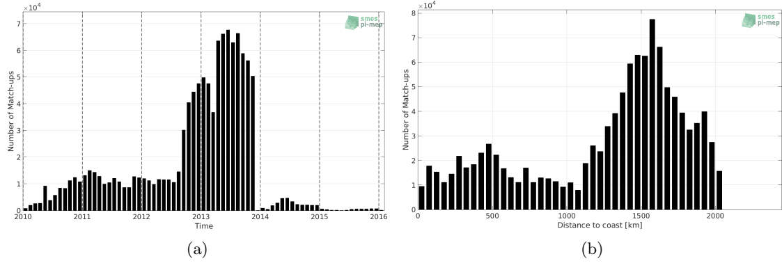
Figure 1: Number of match-ups between Surface drifters and SMOS SSS L3 v4 - 9 Days (CATDS-CECOS-LOCEAN) SSS as a function of time (a) and as function of the distance to coast (b) over the North Atlantic Ocean Pi-MEP region and for the full satellite product period.
