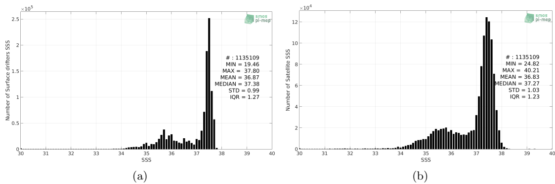
Figure 2: Histograms of SSS from Surface drifters (a) and SMOS SSS L3 v4 - 9 Days (CATDS-CECOS-LOCEAN) (b) considering all match-up pairs per bins of 0.1 over the North Atlantic Ocean Pi-MEP region and for the full satellite product period.
