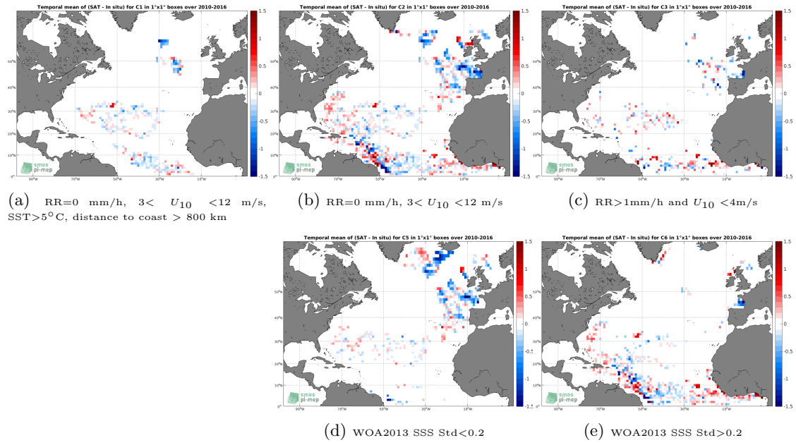
Figure 11: Temporal mean gridded over spatial boxes of size 1^\circ \times 1^\circ of \Delta SSS (SMOS SSS L3 v4 - 9 Days (CATDS-CECOS-LOCEAN) - Surface drifters) for 5 different subdatasets corresponding to: RR=0 mm/h, 3 < U_{10} < 12 m/s, SST > 5^\circ C , distance to coast > 800 km (a), RR=0 mm/h, 3 < U_{10} < 12 m/s (b), RR > 1 mm/h and U_{10} < 4 m/s (c), WOA2013 SSS Std < 0.2 (d), WOA2013 SSS Std > 0.2 (e).
