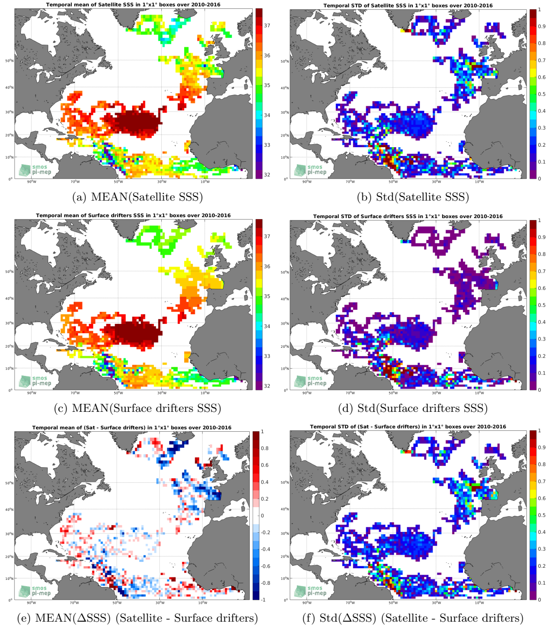
Figure 5: Temporal mean (left) and Std (right) of SSS from SMOS-L3-CATDS-CECOS-LOCEAN-V4-9DAYS-25KM (top), Surface drifters (middle), and of \Delta SSS (Satellite - Surface drifters). Only match-up pairs are used to generate these maps.
