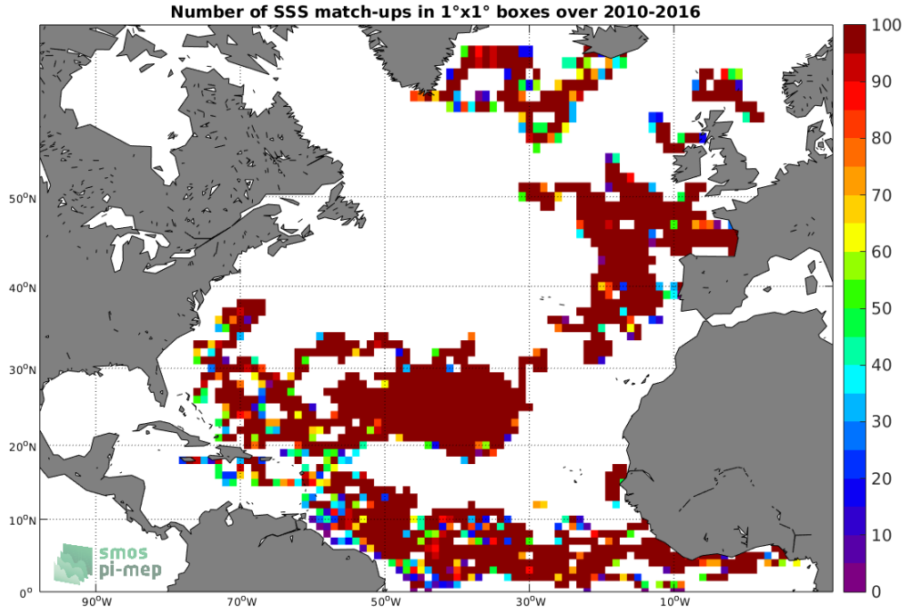
Figure 3: Number of SSS match-ups between Surface drifters SSS and the SMOS-L3-CATDS-CECOS-LOCEAN-V4-9DAYS-25KM SSS product for the North Atlantic Ocean Pi-MEP region over 1^\circ \times 1^\circ boxes and for the full satellite product period.
