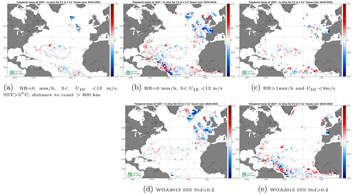
Figure 11: Temporal mean gridded over spatial boxes of size 1^\circ \times 1^\circ of \Delta SSS (SMOS-L3-CATDS-CECOS-LOCEAN-V4-9DAYS-25KM - Surface drifters) for 5 different subdatasets corresponding to:RR=0 mm/h, 3 < U_{10} < 12 m/s, SST >5^\circ\text{C} , distance to coast > 800 km (a), RR=0 mm/h, 3 < U_{10} < 12 m/s (b), RR >1 mm/h and U_{10} < 4 m/s (c), WOA2013 SSS Std <0.2 (d), WOA2013 SSS Std >0.2 (e).
