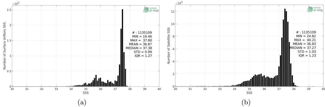
Figure 2: Histograms of SSS from Surface drifters (a) and SMOS-L3-CATDS-CECOS-LOCEAN-V4-9DAYS-25KM (b) considering all match-up pairs per bins of 0.1 over the North Atlantic Ocean Pi-MEP region and for the full satellite product period.
