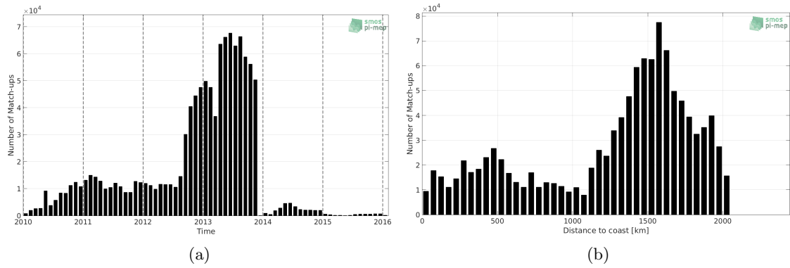
Figure 1: Number of match-ups between Surface drifters and SMOS-L3-CATDS-CECOS-LOCEAN-V4-9DAYS-25KM SSS as a function of time (a) and as function of the distance to coast (b) over the North Atlantic Ocean Pi-MEP region and for the full satellite product period.
