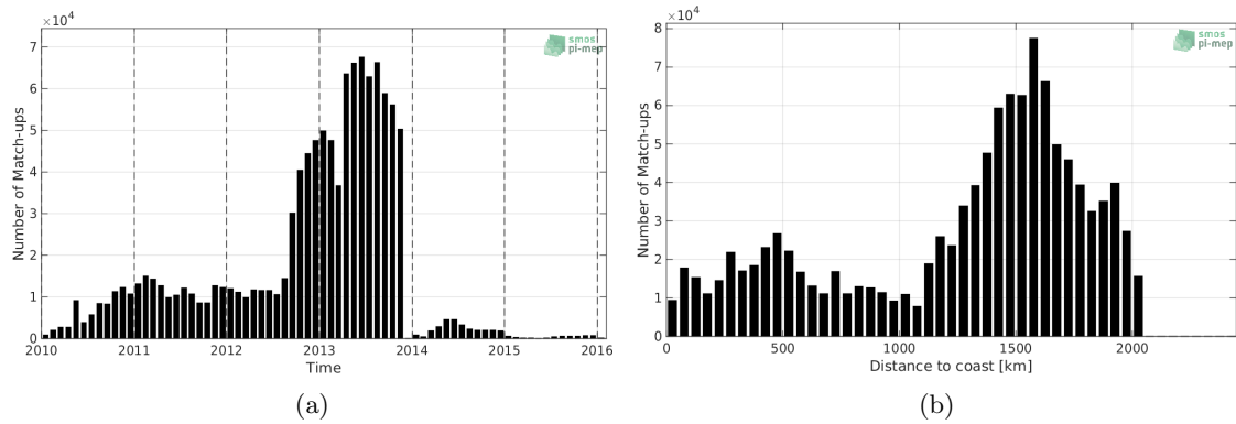
Figure 1: Number of match-ups between Surface drifters and SMOS-L3-CATDS-CECOS-LOCEAN-V4-9DAYS-25KM SSS as a function of time (a) and as function of the distance to coast (b) over the North Atlantic Ocean Pi-MEP region and for the full satellite product period.
