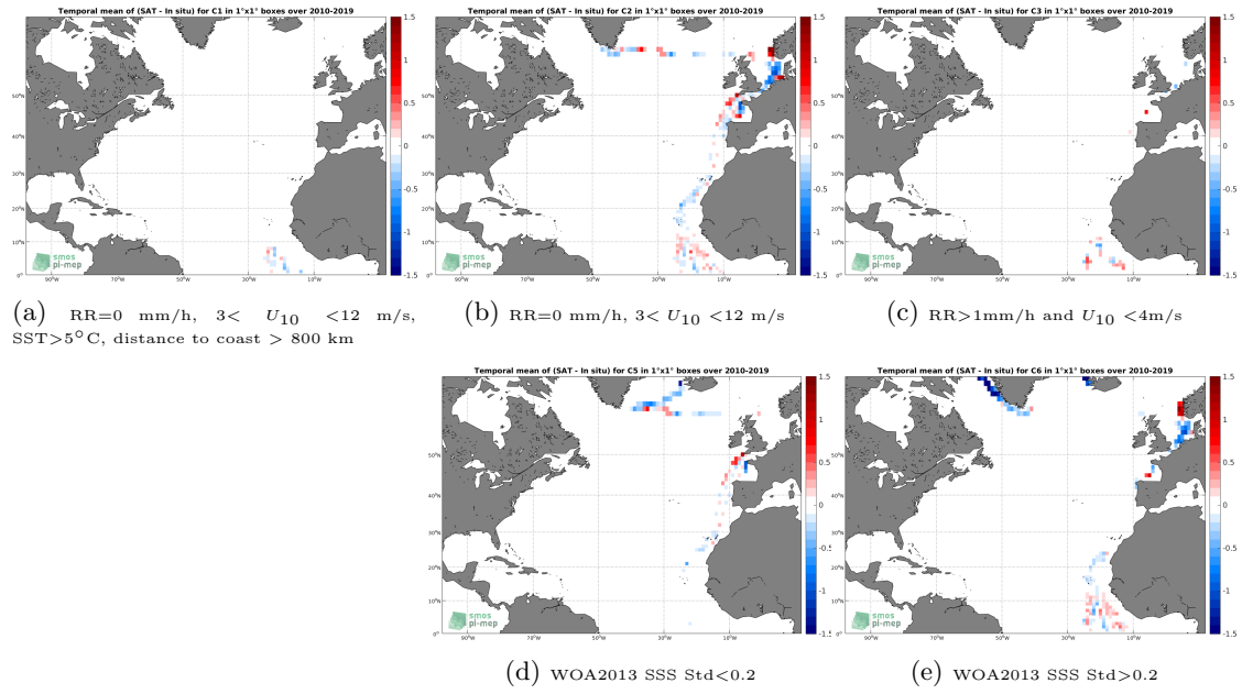
Figure 12: Temporal mean gridded over spatial boxes of size 1^\circ \times 1^\circ of \Delta SSS (SMOS SSS L3 v4 - 18 Days (CATDS-CECOS-LOCEAN) - TSG (Polarstern)) for 5 different subdatasets corresponding to:RR=0 mm/h, 3 < U_{10} < 12 m/s, SST>5°C, distance to coast > 800 km (a), RR=0 mm/h, 3 < U_{10} < 12 m/s (b), RR>1mm/h and U_{10} < 4 m/s (c), WOA2013 SSS Std<0.2 (d), WOA2013 SSS Std>0.2 (e).
