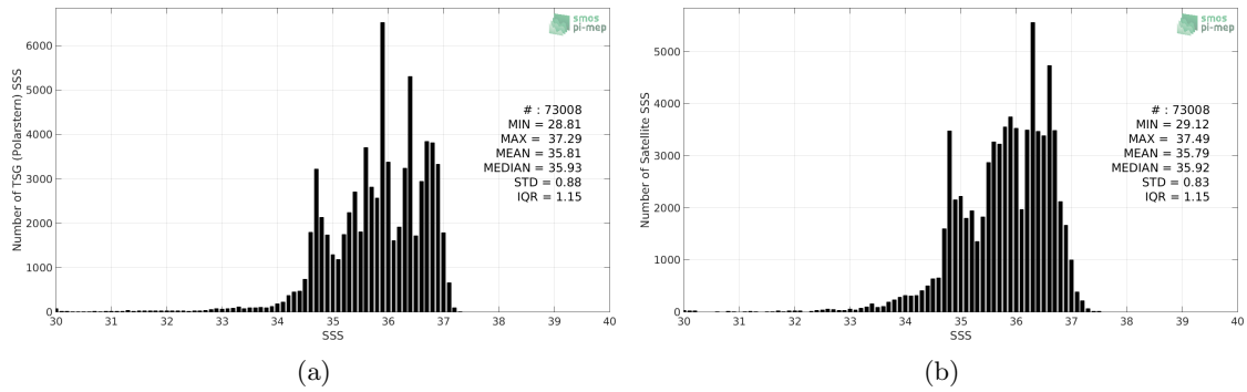
Figure 2: Histograms of SSS from TSG (Polarstern) (a) and SMOS SSS L3 v4 - 18 Days (CATDS-CECOS-LOCEAN) (b) considering all match-up pairs per bins of 0.1 over the North Atlantic Ocean Pi-MEP region and for the full satellite product period.
