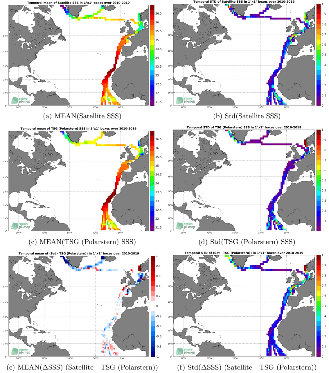
Figure 6: Temporal mean (left) and Std (right) of SSS from SMOS SSS L3 v4 - 18 Days (CATDS-CECOS-LOCEAN) (top), TSG (Polarstern) (middle), and of \Delta SSS (Satellite - TSG (Polarstern)). Only match-up pairs are used to generate these maps.
