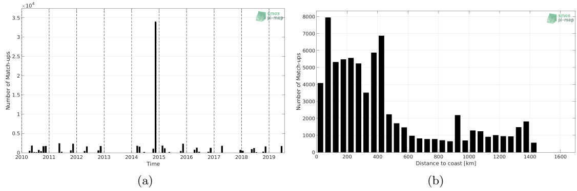
Figure 1: Number of match-ups between TSG (Polarstern) and SMOS SSS L3 v4 - 18 Days (CATDS-CECOS-LOCEAN) SSS as a function of time (a) and as function of the distance to coast (b) over the North Atlantic Ocean Pi-MEP region and for the full satellite product period.
