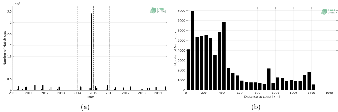
Figure 1: Number of match-ups between TSG-POLARSTERN and SMOS-L3-CATDS-CECOS-LOCEAN-V4-18DAYS-25KM SSS as a function of time (a) and as function of the distance to coast (b) over the North Atlantic Ocean Pi-MEP region and for the full satellite product period.
