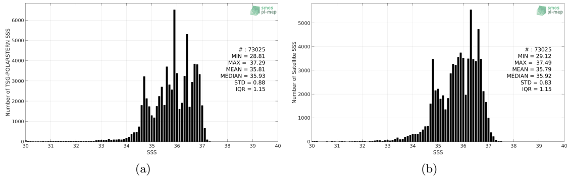
Figure 2: Histograms of SSS from TSG-POLARSTERN (a) and SMOS-L3-CATDS-CECOS-LOCEAN-V4-18DAYS-25KM (b) considering all match-up pairs per bins of 0.1 over the North Atlantic Ocean Pi-MEP region and for the full satellite product period.
