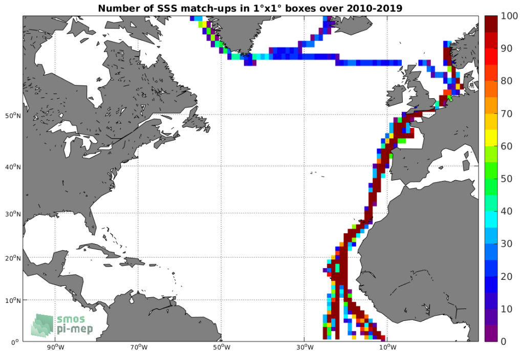
Figure 4: Number of SSS match-ups between TSG-POLARSTERN SSS and the SMOS-L3-CATDS-CECOS-LOCEAN-V4-18DAYS-25KM SSS product for the North Atlantic Ocean Pi-MEP region over 1^\circ \times 1^\circ boxes and for the full satellite product period.
