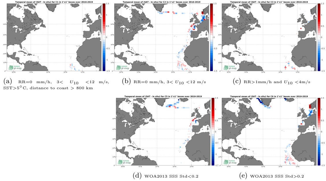
Figure 12: Temporal mean gridded over spatial boxes of size 1^\circ \times 1^\circ of \Delta SSS (SMOS-L3-CATDS-CECOS-LOCEAN-V4-18DAYS-25KM - TSG-POLARSTERN) for 5 different subdatasets corresponding to: RR=0 mm/h, 3 < U_{10} < 12 m/s, SST > 5^\circ\text{C} , distance to coast > 800 km (a), RR=0 mm/h, 3 < U_{10} < 12 m/s (b), RR > 1 mm/h and U_{10} < 4 m/s (c), WOA2013 SSS Std < 0.2 (d), WOA2013 SSS Std > 0.2 (e).
