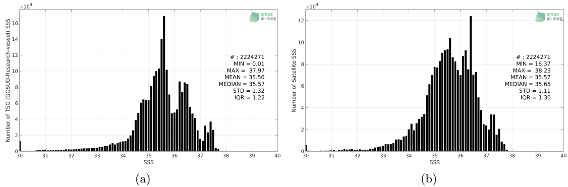
Figure 2: Histograms of SSS from TSG (GOSUD-Research-vessel) (a) and SMOS SSS L3 v4 - 18 Days (CATDS-CECOS-LOCEAN) (b) considering all match-up pairs per bins of 0.1 over the North Atlantic Ocean Pi-MEP region and for the full satellite product period.
