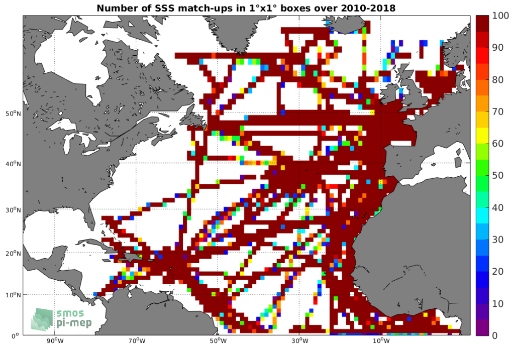
Figure 4: Number of SSS match-ups between TSG (GOSUD-Research-vessel) SSS and the SMOS SSS L3 v4 - 18 Days (CATDS-CECOS-LOCEAN) SSS product for the North Atlantic Ocean Pi-MEP region over 1^\circ \times 1^\circ boxes and for the full satellite product period.
