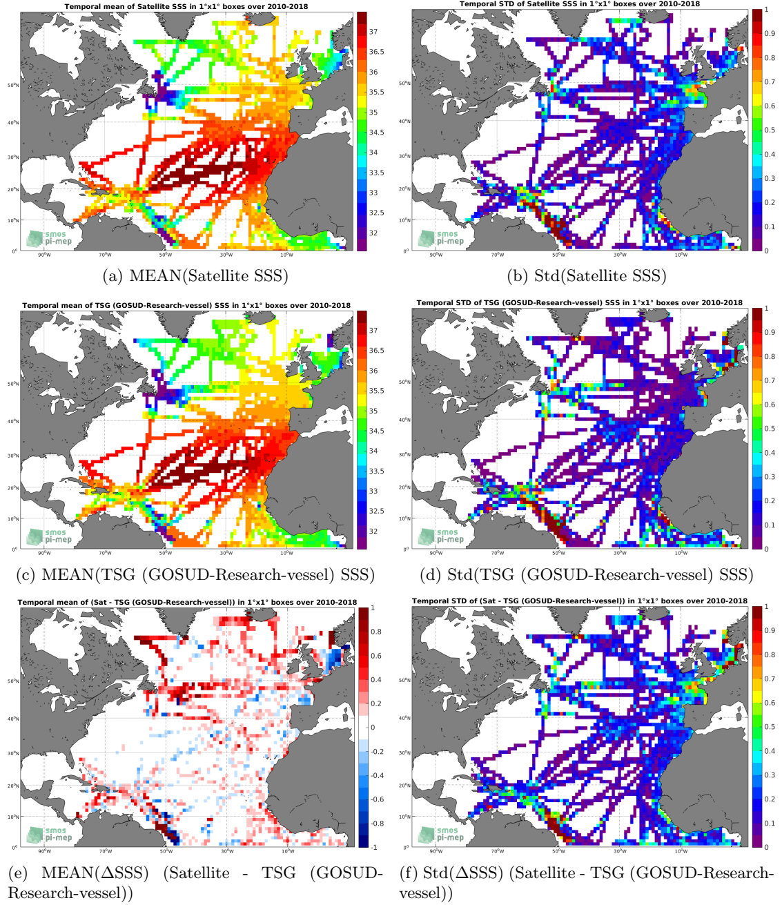
Figure 6: Temporal mean (left) and Std (right) of SSS from SMOS SSS L3 v4 - 18 Days (CATDS-CECOS-LOCEAN) (top), TSG (GOSUD-Research-vessel) (middle), and of \Delta SSS (Satellite - TSG (GOSUD-Research-vessel)). Only match-up pairs are used to generate these maps.
