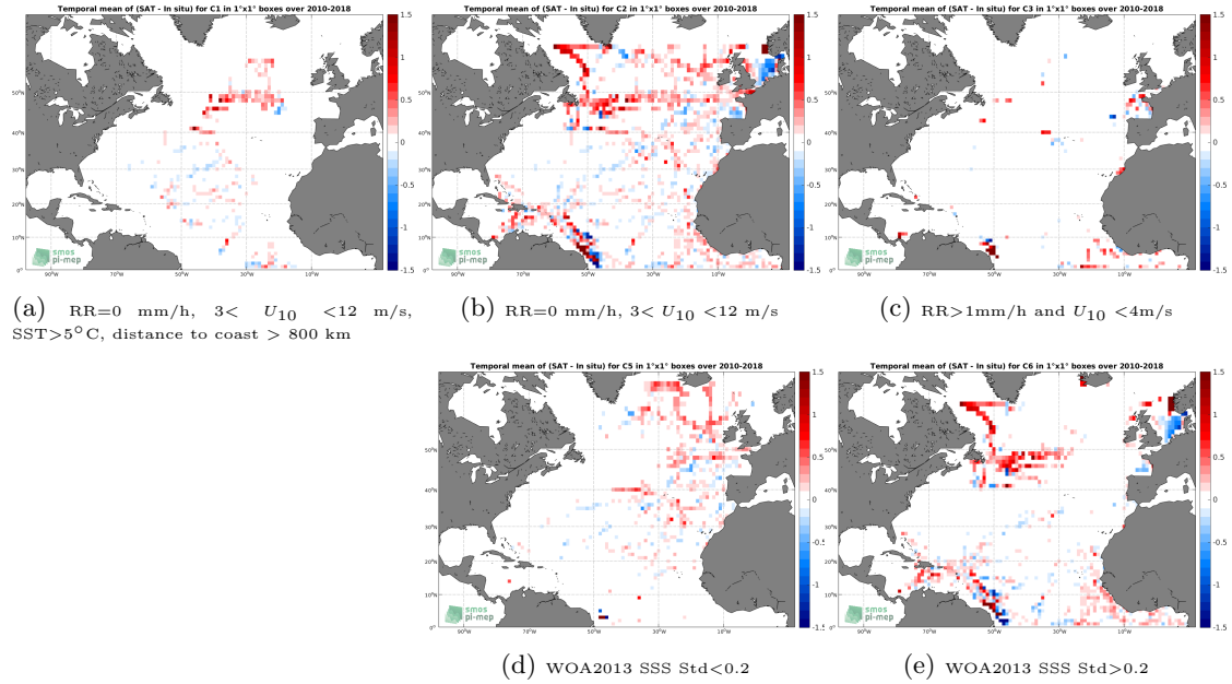
Figure 12: Temporal mean gridded over spatial boxes of size 1^\circ \times 1^\circ of \Delta SSS (SMOS SSS L3 v4 - 18 Days (CATDS-CECOS-LOCEAN) - TSG (GOSUD-Research-vessel)) for 5 different subdatasets corresponding to:RR=0 mm/h, 3 < U_{10} < 12 m/s, SST >5^\circ\text{C} , distance to coast > 800 km (a), RR=0 mm/h, 3 < U_{10} < 12 m/s (b), RR >1 mm/h and U_{10} < 4 m/s (c), WOA2013 SSS Std <0.2 (d), WOA2013 SSS Std >0.2 (e).
