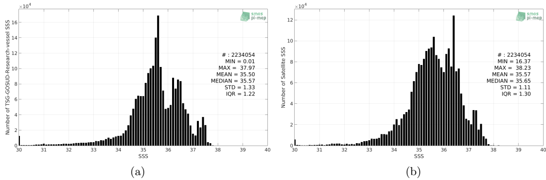
Figure 2: Histograms of SSS from TSG-GOSUD-Research-vessel (a) and SMOS-L3-CATDS-CECOS-LOCEAN-V4-18DAYS-25KM (b) considering all match-up pairs per bins of 0.1 over the North Atlantic Ocean Pi-MEP region and for the full satellite product period.
