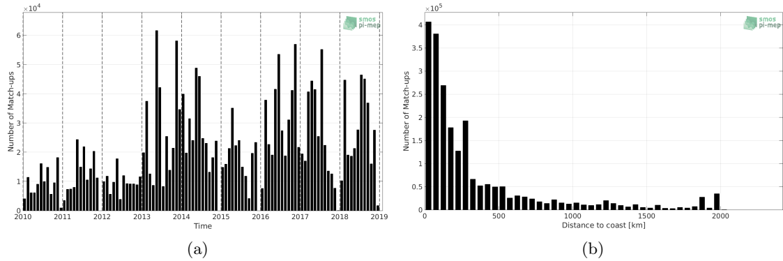
Figure 1: Number of match-ups between TSG-GOSUD-Research-vessel and SMOS-L3-CATDS-CECOS-LOCEAN-V4-18DAYS-25KM SSS as a function of time (a) and as function of the distance to coast (b) over the North Atlantic Ocean Pi-MEP region and for the full satellite product period.
