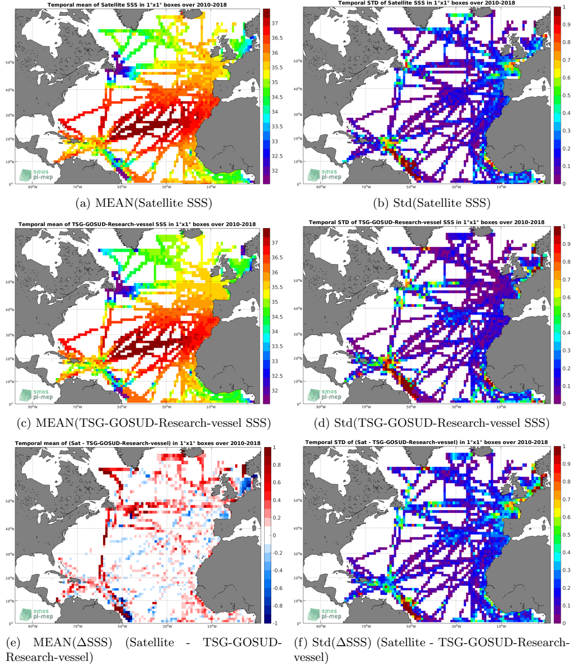
Figure 6: Temporal mean (left) and Std (right) of SSS from SMOS-L3-CATDS-CECOS-LOCEAN-V4-18DAYS-25KM (top), TSG-GOSUD-Research-vessel (middle), and of \Delta SSS (Satellite - TSG-GOSUD-Research-vessel). Only match-up pairs are used to generate these maps.
