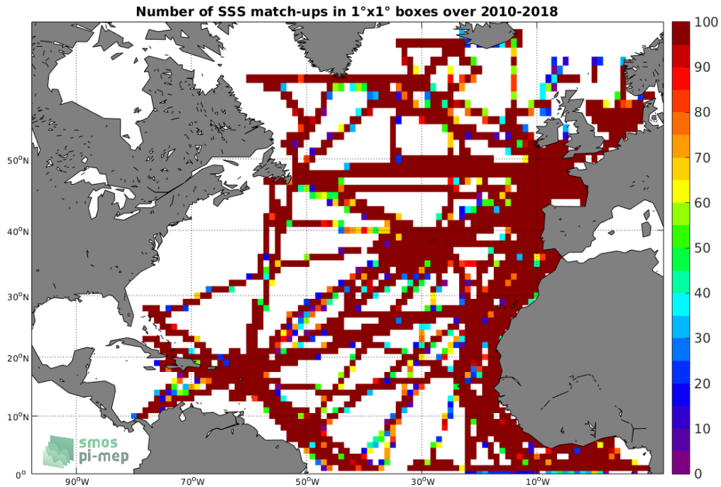
Figure 4: Number of SSS match-ups between TSG-GOSUD-Research-vessel SSS and the SMOS-L3-CATDS-CECOS-LOCEAN-V4-18DAYS-25KM SSS product for the North Atlantic Ocean Pi-MEP region over 1°x1° boxes and for the full satellite product period.
