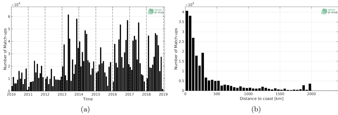
Figure 1: Number of match-ups between TSG-GOSUD-Research-vessel and SMOS-L3-CATDS-CECOS-LOCEAN-V4-18DAYS-25KM SSS as a function of time (a) and as function of the distance to coast (b) over the North Atlantic Ocean Pi-MEP region and for the full satellite product period.
