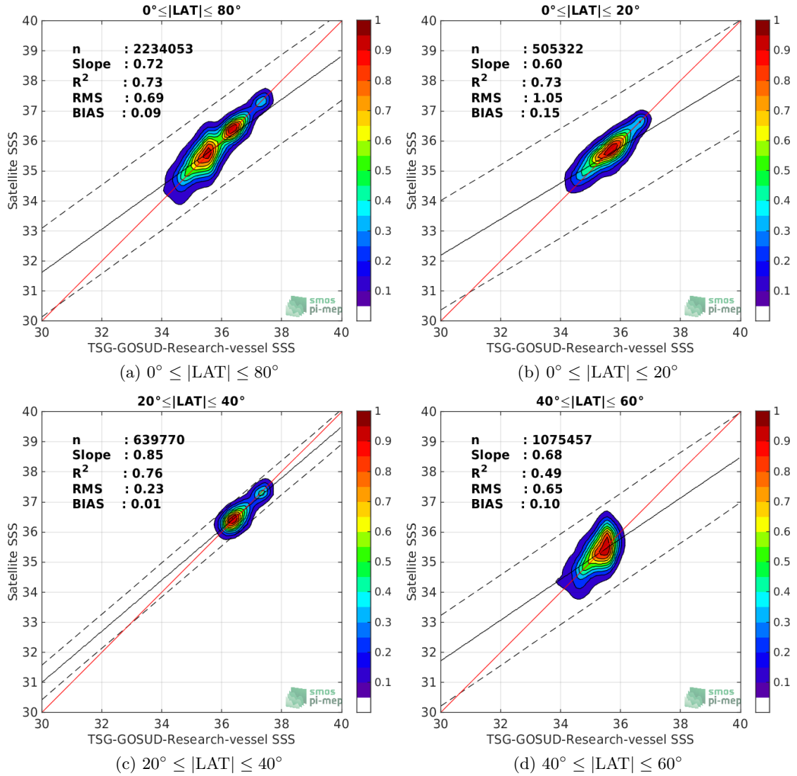
Figure 9: Contour maps of the concentration of SMOS-L3-CATDS-CECOS-LOCEAN-V4-18DAYS-25KM SSS (y-axis) versus TSG-GOSUD-Research-vessel SSS (x-axis) at match-up pairs for different latitude bands. For each plot, the red line shows x=y . The black thin and dashed lines indicate a linear fit through the data cloud and the \pm 95\% confidence levels, respectively. The number match-up pairs n , the slope and R^2 coefficient of the linear fit, the root mean square (RMS) and the mean bias between satellite and in situ data are indicated for each latitude band in each plots.
