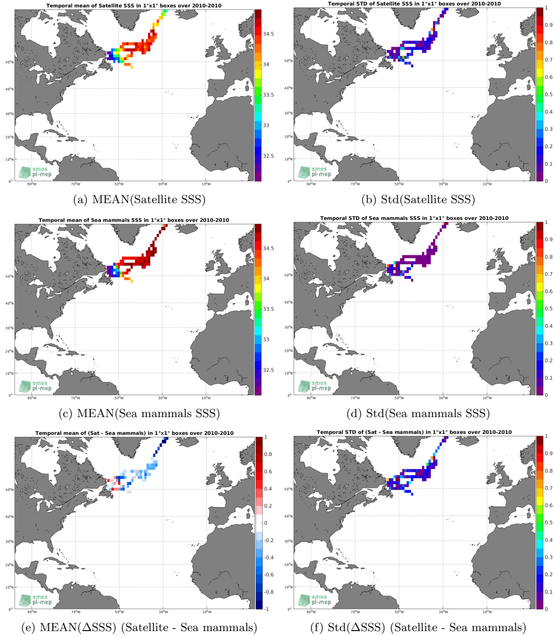
Figure 6: Temporal mean (left) and Std (right) of SSS from SMOS SSS L3 v4 - 18 Days (CATDS-CECOS-LOCEAN) (top), Sea mammals (middle), and of \Delta SSS (Satellite - Sea mammals). Only match-up pairs are used to generate these maps.
