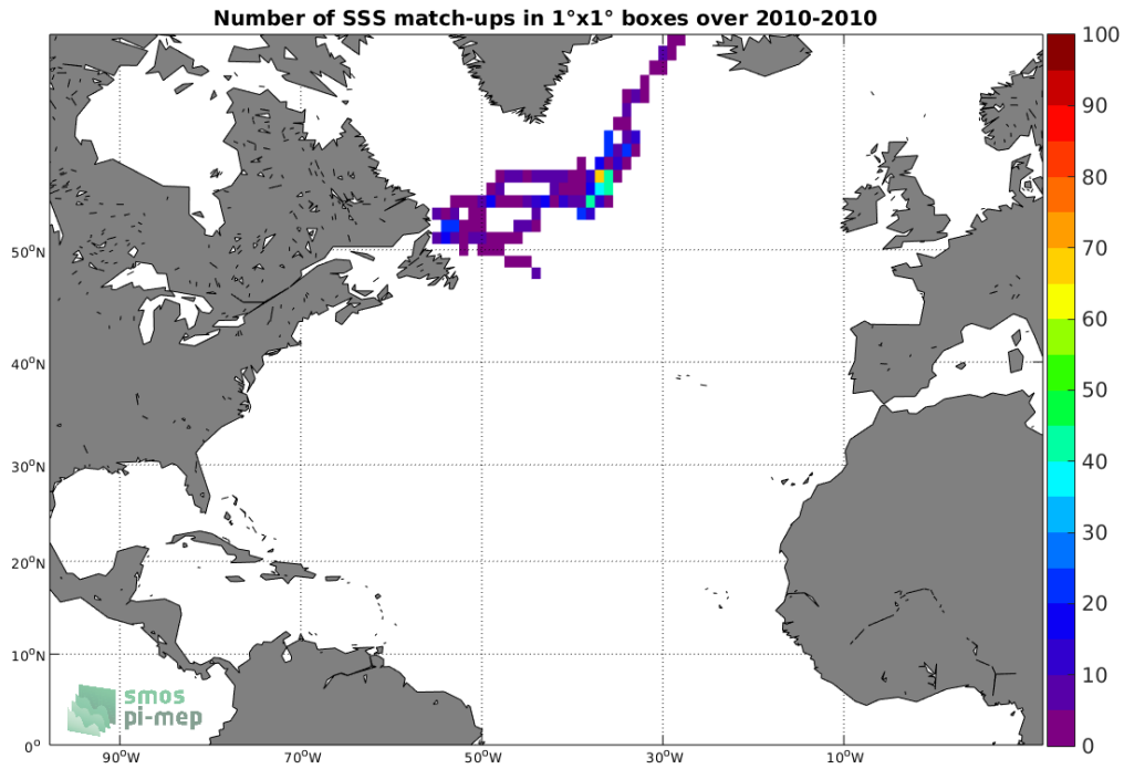
Figure 4: Number of SSS match-ups between Sea mammals SSS and the SMOS SSS L3 v4 - 18 Days (CATDS-CECOS-LOCEAN) SSS product for the North Atlantic Ocean Pi-MEP region over 1°x1° boxes and for the full satellite product period.
