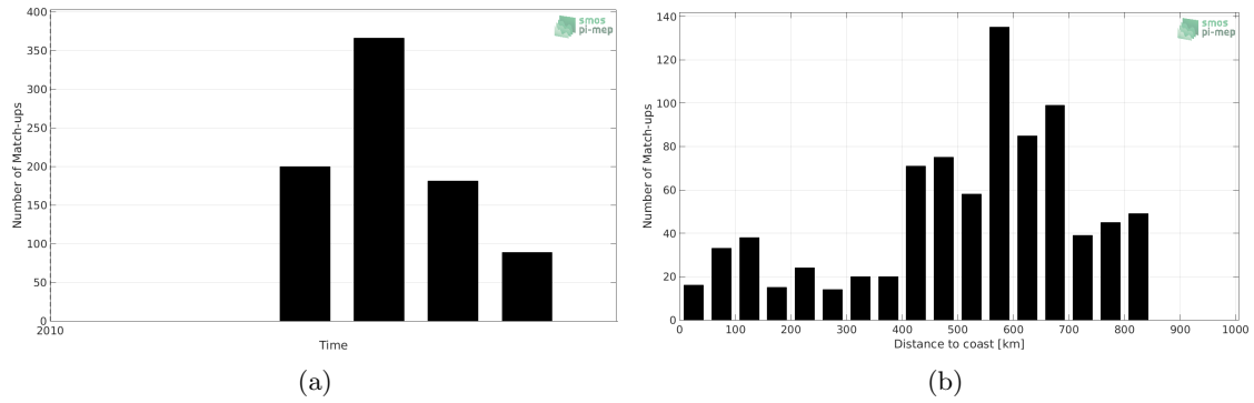
Figure 1: Number of match-ups between Sea mammals and SMOS SSS L3 v4 - 18 Days (CATDS-CECOS-LOCEAN) SSS as a function of time (a) and as function of the distance to coast (b) over the North Atlantic Ocean Pi-MEP region and for the full satellite product period.
