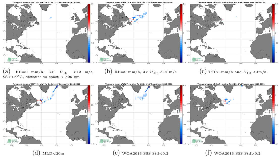
Figure 12: Temporal mean gridded over spatial boxes of size 1^{\circ}\times 1^{\circ} of \Delta\text{SSS} (SMOS SSS L3 v4 - 18 Days (CATDS-CECOS-LOCEAN) - Sea mammals) for 6 different subdatasets corresponding to:RR=0 mm/h, 3 < U_{10} < 12 m/s, SST >5^{\circ}\text{C} , distance to coast > 800 km (a), RR=0 mm/h, 3 < U_{10} < 12 m/s (b), RR >1\text{mm/h} and U_{10} < 4\text{m/s} (c),MLD <20\text{m} (d),WOA2013 SSS Std <0.2 (e),WOA2013 SSS Std >0.2 (f).
