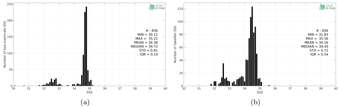
Figure 2: Histograms of SSS from Sea mammals (a) and SMOS SSS L3 v4 - 18 Days (CATDS-CECOS-LOCEAN) (b) considering all match-up pairs per bins of 0.1 over the North Atlantic Ocean Pi-MEP region and for the full satellite product period.
