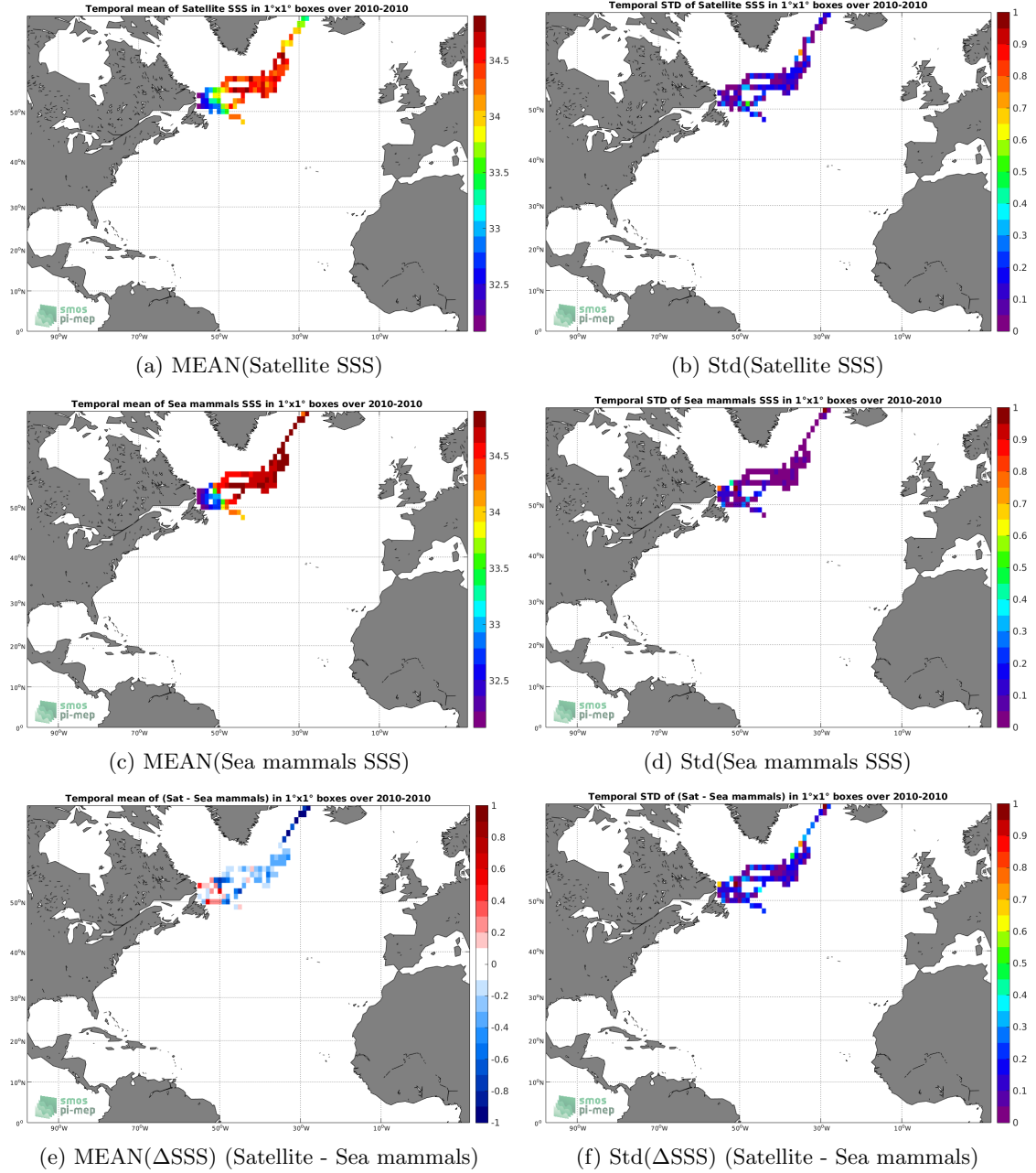
Figure 6: Temporal mean (left) and Std (right) of SSS from SMOS-L3-CATDS-CECOS-LOCEAN-V4-18DAYS-25KM (top), Sea mammals (middle), and of \Delta SSS (Satellite - Sea mammals). Only match-up pairs are used to generate these maps.
