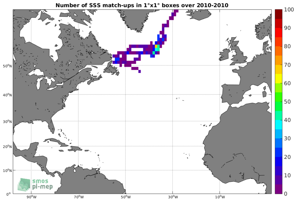
Figure 4: Number of SSS match-ups between Sea mammals SSS and the SMOS-L3-CATDS-CECOS-LOCEAN-V4-18DAYS-25KM SSS product for the North Atlantic Ocean Pi-MEP region over 1^\circ \times 1^\circ boxes and for the full satellite product period.
