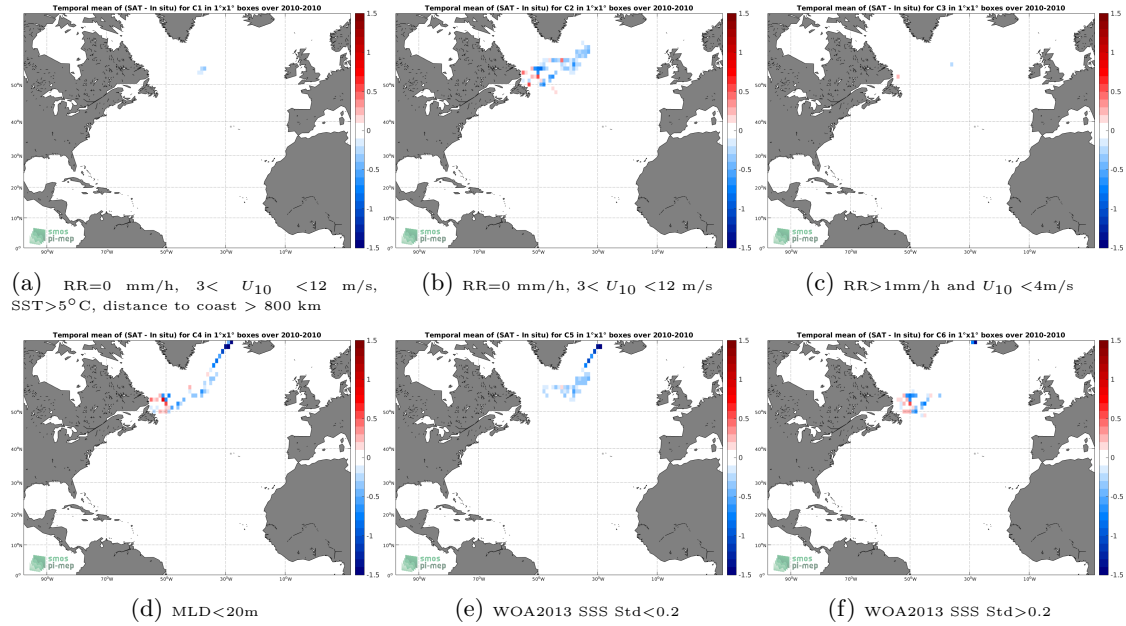
Figure 12: Temporal mean gridded over spatial boxes of size 1^{\circ}\times 1^{\circ} of \Delta\text{SSS} (SMOS-L3-CATDS-CECOS-LOCEAN-V4-18DAYS-25KM - Sea mammals) for 6 different subdatasets corresponding to:RR=0 mm/h, 3 < U_{10} < 12 m/s, SST >5^{\circ}\text{C} , distance to coast > 800 km (a), RR=0 mm/h, 3 < U_{10} < 12 m/s (b), RR >1\text{mm/h} and U_{10} < 4\text{m/s} (c),MLD <20\text{m} (d),WOA2013 SSS Std <0.2 (e),WOA2013 SSS Std >0.2 (f).
