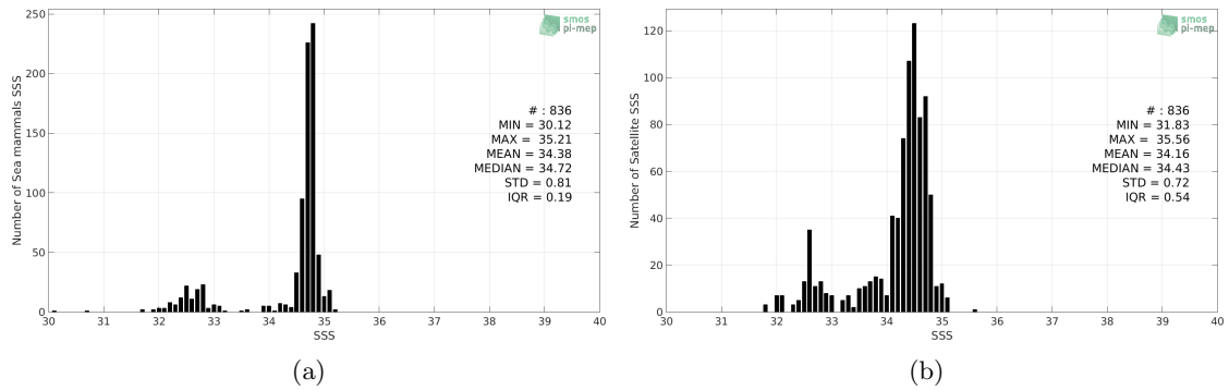
Figure 2: Histograms of SSS from Sea mammals (a) and SMOS-L3-CATDS-CECOS-LOCEAN-V4-18DAYS-25KM (b) considering all match-up pairs per bins of 0.1 over the North Atlantic Ocean Pi-MEP region and for the full satellite product period.
