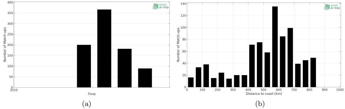
Figure 1: Number of match-ups between Sea mammals and SMOS-L3-CATDS-CECOS-LOCEAN-V4-18DAYS-25KM SSS as a function of time (a) and as function of the distance to coast (b) over the North Atlantic Ocean Pi-MEP region and for the full satellite product period.
