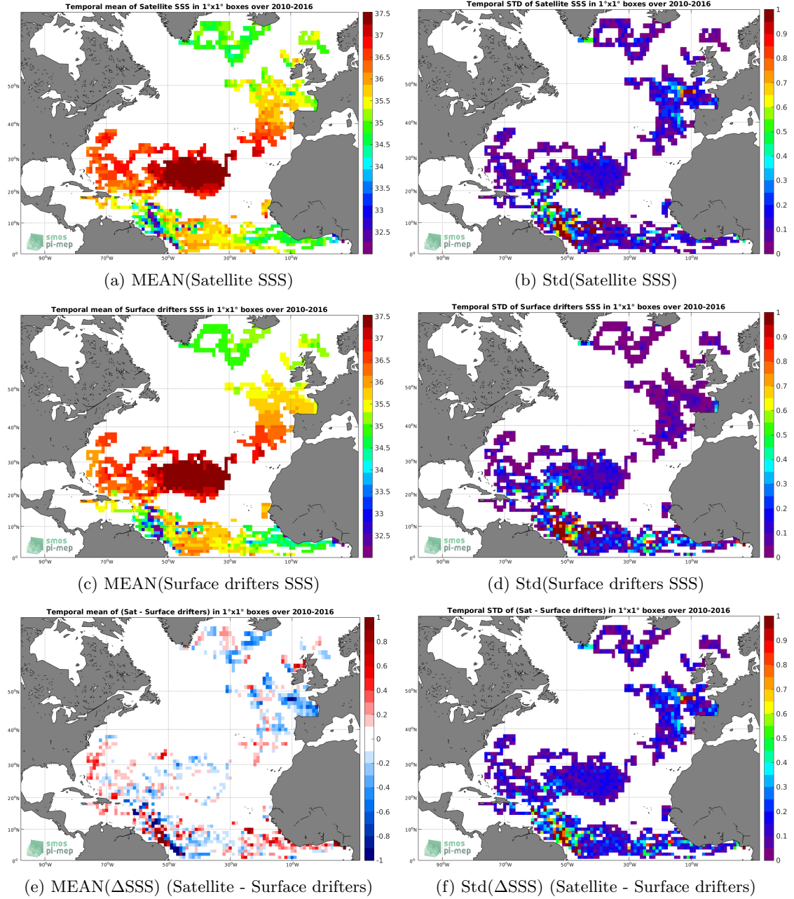
Figure 5: Temporal mean (left) and Std (right) of SSS from SMOS-L3-CATDS-CECOS-LOCEAN-V4-18DAYS-25KM (top), Surface drifters (middle), and of \Delta SSS (Satellite - Surface drifters). Only match-up pairs are used to generate these maps.
