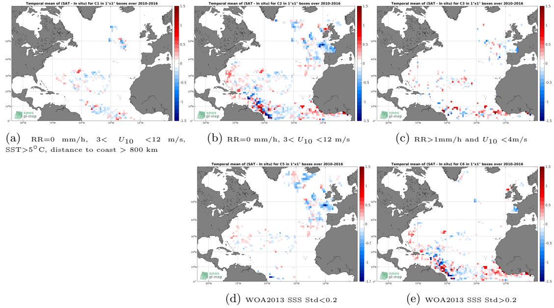
Figure 11: Temporal mean gridded over spatial boxes of size 1^\circ \times 1^\circ of \Delta SSS (SMOS-L3-CATDS-CECOS-LOCEAN-V4-18DAYS-25KM - Surface drifters) for 5 different subdatasets corresponding to: RR=0 mm/h, 3 < U_{10} < 12 m/s, SST >5^\circ\text{C} , distance to coast > 800 km (a), RR=0 mm/h, 3 < U_{10} < 12 m/s (b), RR >1 mm/h and U_{10} < 4 m/s (c), WOA2013 SSS Std <0.2 (d), WOA2013 SSS Std >0.2 (e).
