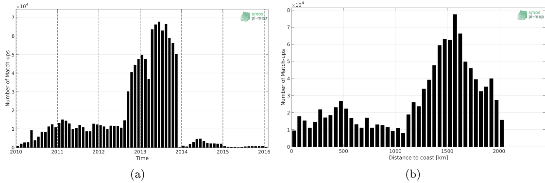
Figure 1: Number of match-ups between Surface drifters and SMOS-L3-CATDS-CECOS-LOCEAN-V4-18DAYS-25KM SSS as a function of time (a) and as function of the distance to coast (b) over the North Atlantic Ocean Pi-MEP region and for the full satellite product period.
