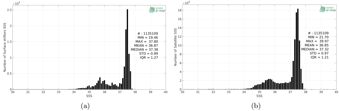
Figure 2: Histograms of SSS from Surface drifters (a) and SMOS-L3-CATDS-CECOS-LOCEAN-V4-18DAYS-25KM (b) considering all match-up pairs per bins of 0.1 over the North Atlantic Ocean Pi-MEP region and for the full satellite product period.
