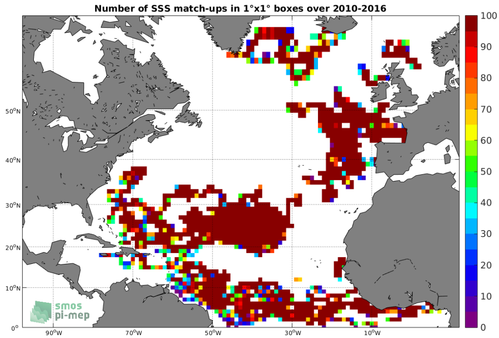
Figure 3: Number of SSS match-ups between Surface drifters SSS and the SMOS-L3-CATDS-CECOS-LOCEAN-V4-18DAYS-25KM SSS product for the North Atlantic Ocean Pi-MEP region over 1°x1° boxes and for the full satellite product period.
