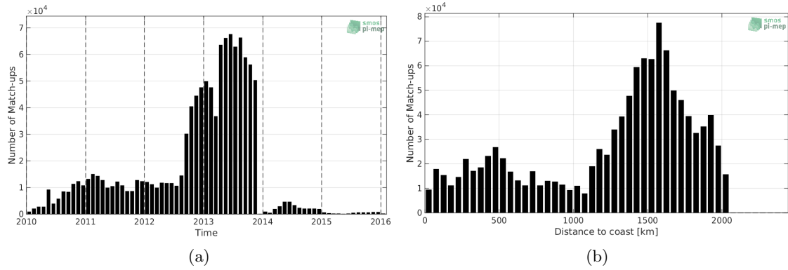
Figure 1: Number of match-ups between Surface drifters and SMOS-L3-CATDS-CECOS-LOCEAN-V4-18DAYS-25KM SSS as a function of time (a) and as function of the distance to coast (b) over the North Atlantic Ocean Pi-MEP region and for the full satellite product period.
