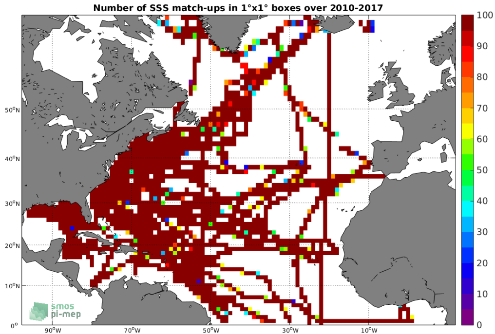
Figure 4: Number of SSS match-ups between TSG-SAMOS SSS and the SMOS-L3-CATDS-CECOS-LOCEAN-V3-9DAYS-25KM SSS product for the North Atlantic Ocean Pi-MEP region over 1^\circ \times 1^\circ boxes and for the full satellite product period.
