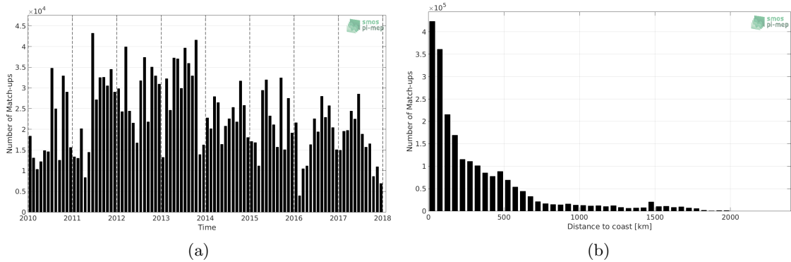
Figure 1: Number of match-ups between TSG-LEGOS-DM and SMOS-L3-CATDS-CECOS-LOCEAN-V3-9DAYS-25KM SSS as a function of time (a) and as function of the distance to coast (b) over the North Atlantic Ocean Pi-MEP region and for the full satellite product period.
