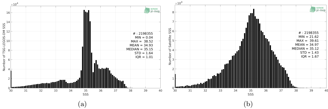
Figure 2: Histograms of SSS from TSG-LEGOS-DM (a) and SMOS-L3-CATDS-CECOS-LOCEAN-V3-9DAYS-25KM (b) considering all match-up pairs per bins of 0.1 over the North Atlantic Ocean Pi-MEP region and for the full satellite product period.
