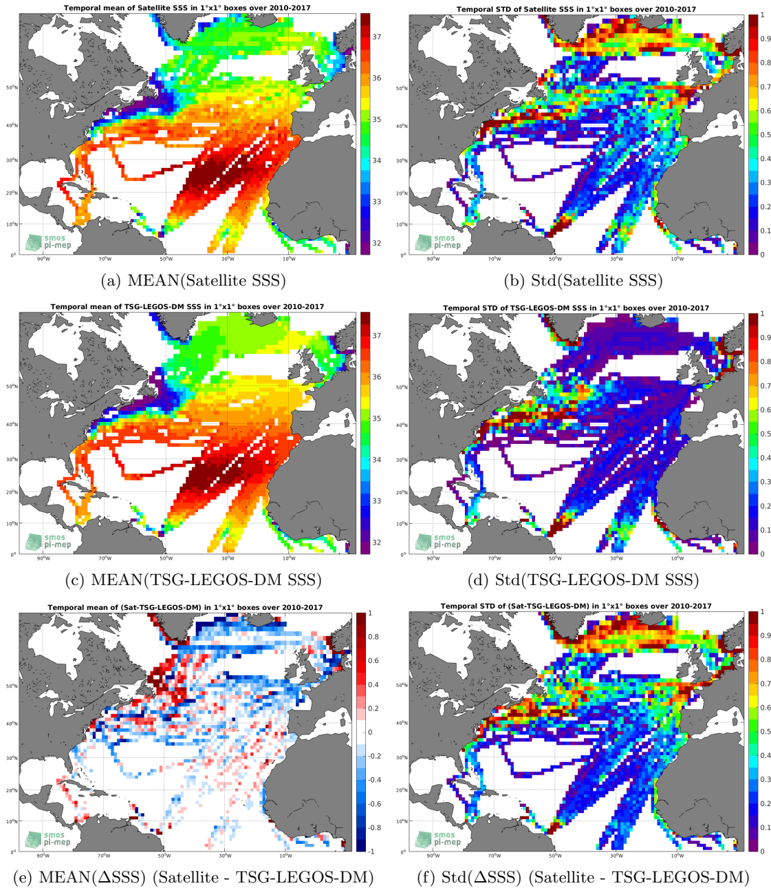
Figure 6: Temporal mean (left) and Std (right) of SSS from SMOS-L3-CATDS-CECOS-LOCEAN-V3-9DAYS-25KM (top), TSG-LEGOS-DM (middle), and of \Delta SSS (Satellite - TSG-LEGOS-DM). Only match-up pairs are used to generate these maps.
