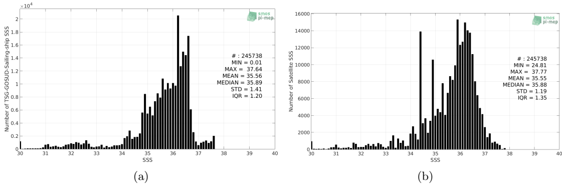
Figure 2: Histograms of SSS from TSG-GOSUD-Sailing-ship (a) and SMOS-L3-CATDS-CECOS-LOCEAN-V3-9DAYS-25KM (b) considering all match-up pairs per bins of 0.1 over the North Atlantic Ocean Pi-MEP region and for the full satellite product period.
