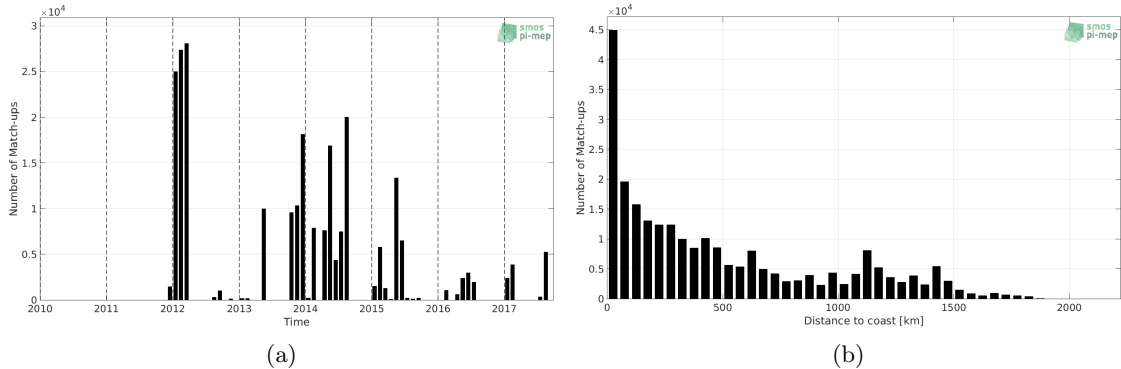
Figure 1: Number of match-ups between TSG-GOSUD-Sailing-ship and SMOS-L3-CATDS-CECOS-LOCEAN-V3-9DAYS-25KM SSS as a function of time (a) and as function of the distance to coast (b) over the North Atlantic Ocean Pi-MEP region and for the full satellite product period.
