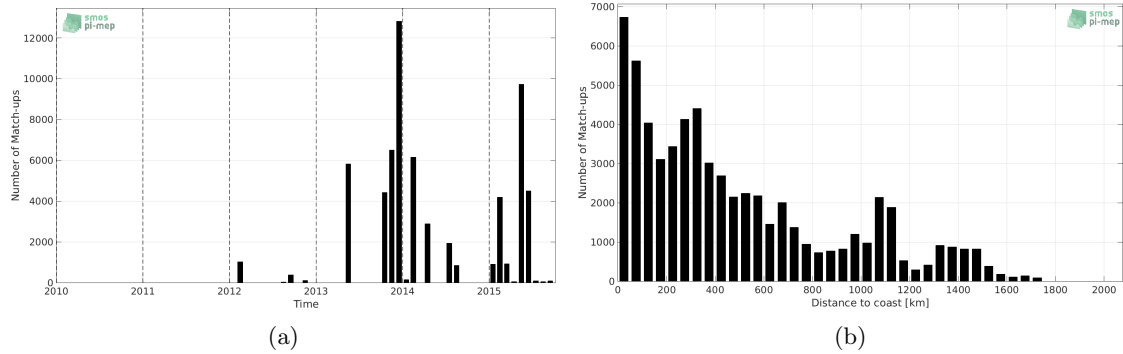
Figure 1: Number of match-ups between TSG-GOSUD-Sailing-ship and SMOS-L3-CATDS-CECOS-LOCEAN-V3-9DAYS-25KM SSS as a function of time (a) and as function of the distance to coast (b) over the North Atlantic Ocean Pi-MEP region and for the full satellite product period.
