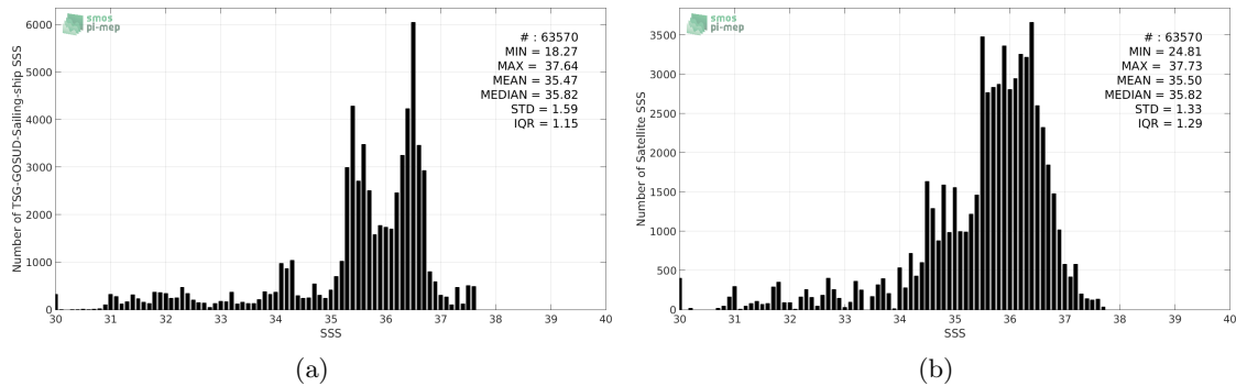
Figure 2: Histograms of SSS from TSG-GOSUD-Sailing-ship (a) and SMOS-L3-CATDS-CECOS-LOCEAN-V3-9DAYS-25KM (b) considering all match-up pairs per bins of 0.1 over the North Atlantic Ocean Pi-MEP region and for the full satellite product period.
