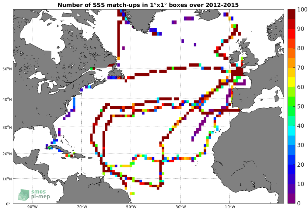
Figure 4: Number of SSS match-ups between TSG-GOSUD-Sailing-ship SSS and the SMOS-L3-CATDS-CECOS-LOCEAN-V3-9DAYS-25KM SSS product for the North Atlantic Ocean Pi-MEP region over 1^\circ \times 1^\circ boxes and for the full satellite product period.
