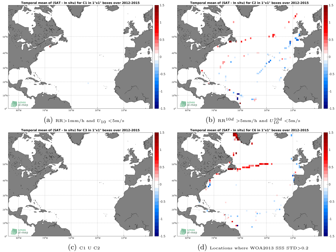
Figure 12: Temporal mean gridded over spatial boxes of size 1^\circ \times 1^\circ of \Delta SSS (SMOS-L3-CATDS-CECOS-LOCEAN-V3-9DAYS-25KM - TSG-GOSUD-Sailing-ship) for 4 different subdatasets corresponding to:RR >1\text{mm/h} and U_{10} < 5\text{m/s} (a), RR^{10d} > 5\text{mm/h} and U_{10}^{10d} < 5\text{m/s} (b), C1 U C2 (c),Locations where WOA2013 SSS STD >0.2 (d).
