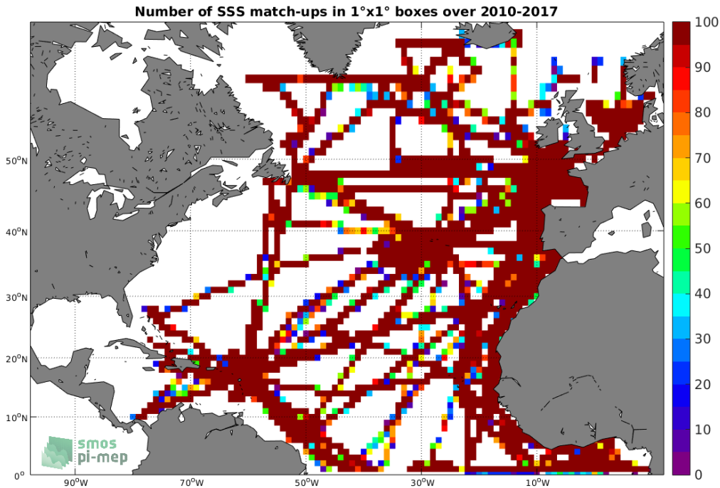
Figure 4: Number of SSS match-ups between TSG-GOSUD-Research-vessel SSS and the SMOS-L3-CATDS-CECOS-LOCEAN-V3-9DAYS-25KM SSS product for the North Atlantic Ocean Pi-MEP region over 1°x1° boxes and for the full satellite product period.
