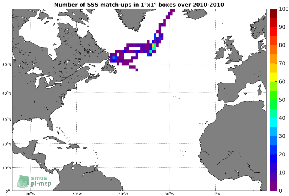
Figure 4: Number of SSS match-ups between Sea mammals SSS and the SMOS-L3-CATDS-CECOS-LOCEAN-V3-9DAYS-25KM SSS product for the North Atlantic Ocean Pi-MEP region over 1^\circ \times 1^\circ boxes and for the full satellite product period.
