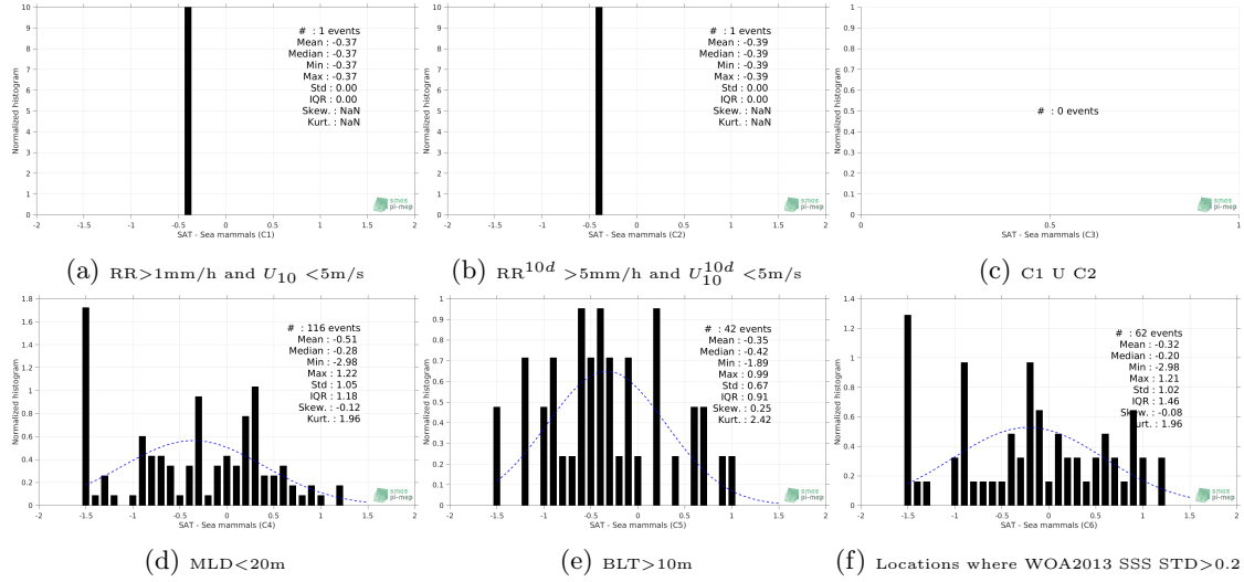
Figure 13: Normalized histogram of \Delta SSS (SMOS-L3-CATDS-CECOS-LOCEAN-V3-9DAYS-25KM - Sea mammals) for 6 different subdatasets corresponding to: RR>1mm/h and U_{10} < 5 m/s (a), RR 10d >5mm/h and U_{10}^{10d} < 5 m/s (b), C1 U C2 (c),MLD<20m (d),BLT>10m (e),Locations where WOA2013 SSS STD>0.2 (f).
