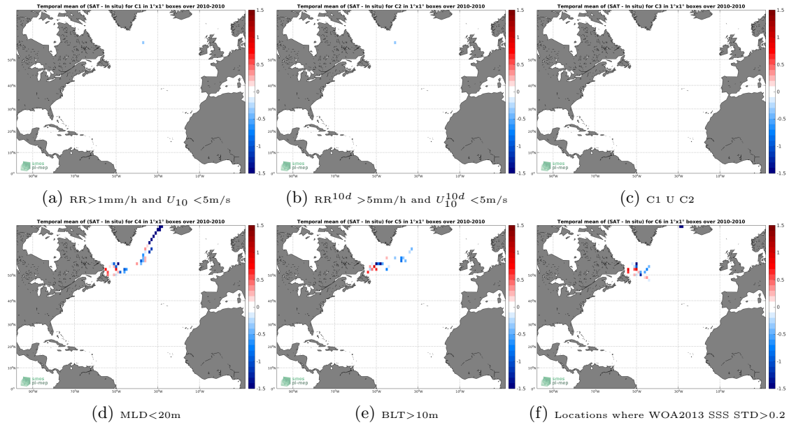
Figure 12: Temporal mean gridded over spatial boxes of size 1^\circ \times 1^\circ of \Delta\text{SSS} (SMOS-L3-CATDS-CECOS-LOCEAN-V3-9DAYS-25KM - Sea mammals) for 6 different subdatasets corresponding to: \text{RR} > 1\text{mm/h} and U_{10} < 5\text{m/s} (a), \text{RR}^{10d} > 5\text{mm/h} and U_{10}^{10d} < 5\text{m/s} (b), C1 U C2 (c), \text{MLD} < 20\text{m} (d), \text{BLT} > 10\text{m} (e), Locations where WOA2013 SSS STD > 0.2 (f).
