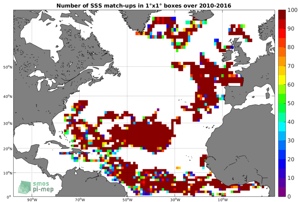
Figure 3: Number of SSS match-ups between Surface drifters SSS and the SMOS-L3-CATDS-CECOS-LOCEAN-V3-9DAYS-25KM SSS product for the North Atlantic Ocean Pi-MEP region over 1^\circ \times 1^\circ boxes and for the full satellite product period.
