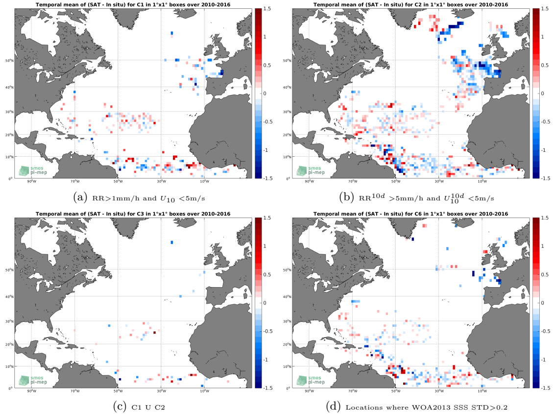
Figure 11: Temporal mean gridded over spatial boxes of size 1^\circ \times 1^\circ of \Delta SSS (SMOS-L3-CATDS-CECOS-LOCEAN-V3-9DAYS-25KM - Surface drifters) for 4 different subdatasets corresponding to: RR > 1\text{mm/h} and U_{10} < 5\text{m/s} (a), RR^{10d} > 5\text{mm/h} and U_{10}^{10d} < 5\text{m/s} (b), C1 U C2 (c), Locations where WOA2013 SSS STD > 0.2 (d).
