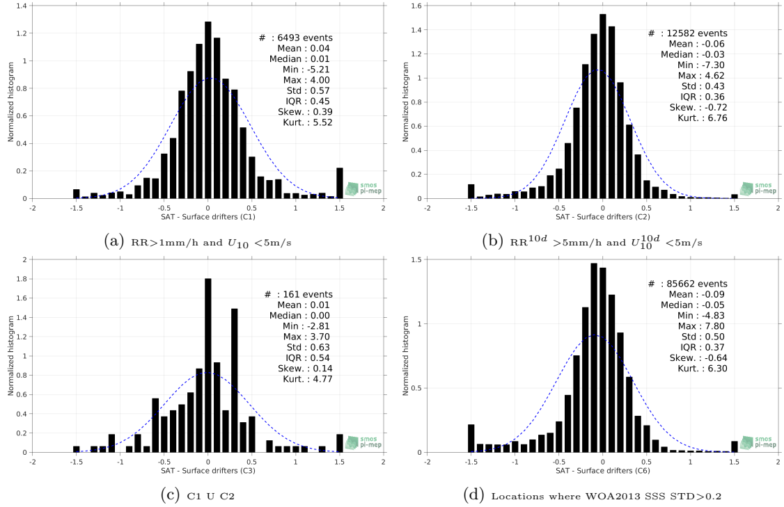
Figure 12: Normalized histogram of \Delta SSS (SMOS-L3-CATDS-CECOS-LOCEAN-V3-9DAYS-25KM - Surface drifters) for 6 different subdatasets corresponding to: RR > 1mm/h and U_{10} < 5 m/s (a), RR^{10d} > 5 mm/h and U_{10}^{10d} < 5 m/s (b), C1 U C2 (c), Locations where WOA2013 SSS STD > 0.2 (d).
