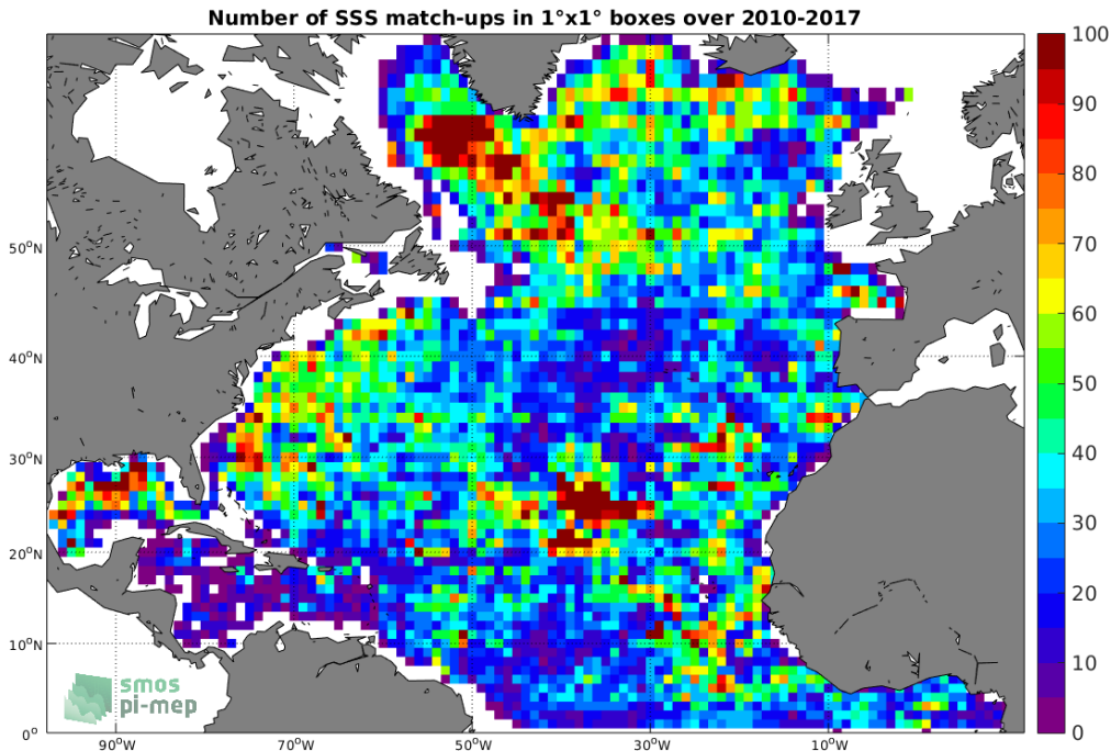
Figure 4: Number of SSS match-ups between Argo SSS and the SMOS-L3-CATDS-CECOS-LOCEAN-V3-9DAYS-25KM SSS product for the North Atlantic Ocean Pi-MEP region over 1^\circ \times 1^\circ boxes and for the full satellite product period.
