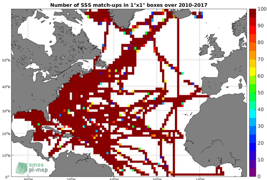
Figure 4: Number of SSS match-ups between TSG-SAMOS SSS and the SMOS-L3-CATDS-CECOS-LOCEAN-V3-18DAYS-25KM SSS product for the North Atlantic Ocean Pi-MEP region over 1°x1° boxes and for the full satellite product period.
