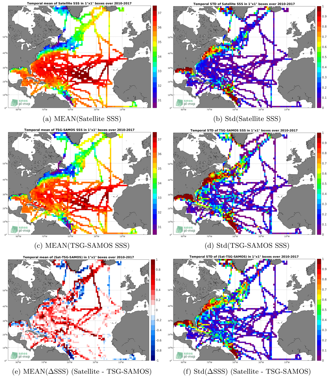
Figure 6: Temporal mean (left) and Std (right) of SSS from SMOS-L3-CATDS-CECOS-LOCEAN-V3-18DAYS-25KM (top), TSG-SAMOS (middle), and of \Delta SSS (Satellite - TSG-SAMOS). Only match-up pairs are used to generate these maps.
