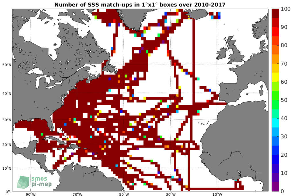
Figure 4: Number of SSS match-ups between TSG-SAMOS SSS and the SMOS-L3-CATDS-CECOS-LOCEAN-V3-18DAYS-25KM SSS product for the North Atlantic Ocean Pi-MEP region over 1^\circ \times 1^\circ boxes and for the full satellite product period.
