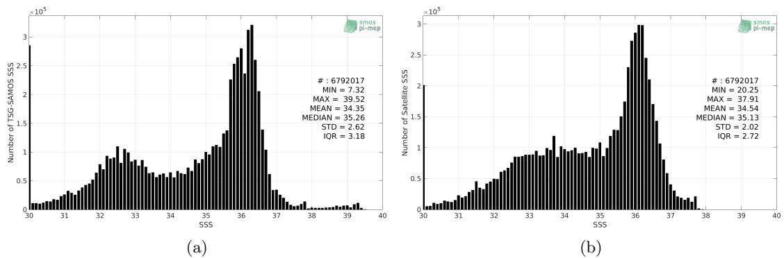
Figure 2: Histograms of SSS from TSG-SAMOS (a) and SMOS-L3-CATDS-CECOS-LOCEAN-V3-18DAYS-25KM (b) considering all match-up pairs per bins of 0.1 over the North Atlantic Ocean Pi-MEP region and for the full satellite product period.
