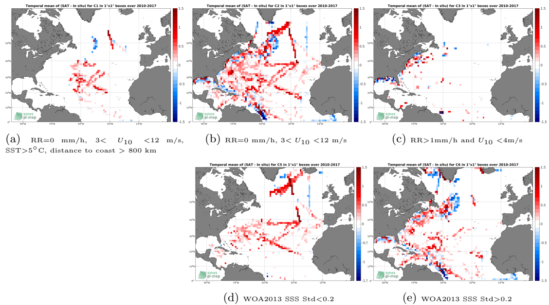
Figure 12: Temporal mean gridded over spatial boxes of size 1^\circ \times 1^\circ of \Delta SSS (SMOS-L3-CATDS-CECOS-LOCEAN-V3-18DAYS-25KM - TSG-SAMOS) for 5 different subdatasets corresponding to:RR=0 mm/h, 3 < U_{10} < 12 m/s, SST >5^\circ C, distance to coast > 800 km (a), RR=0 mm/h, 3 < U_{10} < 12 m/s (b), RR >1 mm/h and U_{10} < 4 m/s (c), WOA2013 SSS Std <0.2 (d), WOA2013 SSS Std >0.2 (e).
