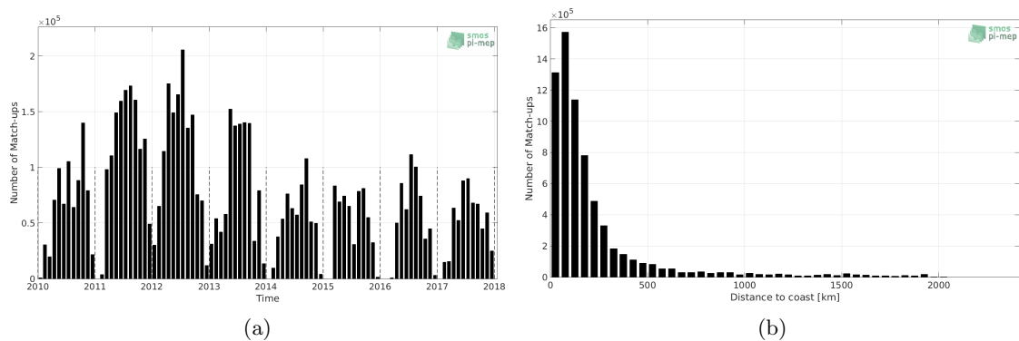
Figure 1: Number of match-ups between TSG-SAMOS and SMOS-L3-CATDS-CECOS-LOCEAN-V3-18DAYS-25KM SSS as a function of time (a) and as function of the distance to coast (b) over the North Atlantic Ocean Pi-MEP region and for the full satellite product period.
