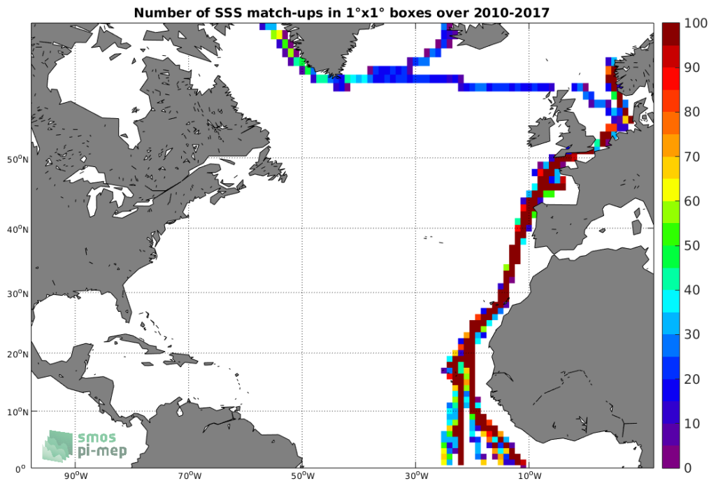
Figure 4: Number of SSS match-ups between TSG-POLARSTERN SSS and the SMOS-L3-CATDS-CECOS-LOCEAN-V3-18DAYS-25KM SSS product for the North Atlantic Ocean Pi-MEP region over 1°x1° boxes and for the full satellite product period.
