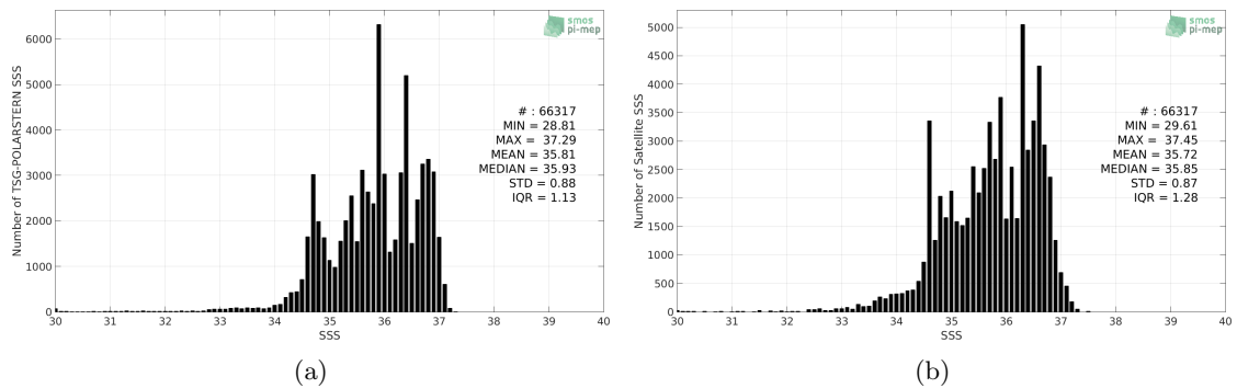
Figure 2: Histograms of SSS from TSG-POLARSTERN (a) and SMOS-L3-CATDS-CECOS-LOCEAN-V3-18DAYS-25KM (b) considering all match-up pairs per bins of 0.1 over the North Atlantic Ocean Pi-MEP region and for the full satellite product period.
