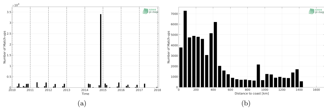
Figure 1: Number of match-ups between TSG-POLARSTERN and SMOS-L3-CATDS-CECOS-LOCEAN-V3-18DAYS-25KM SSS as a function of time (a) and as function of the distance to coast (b) over the North Atlantic Ocean Pi-MEP region and for the full satellite product period.
