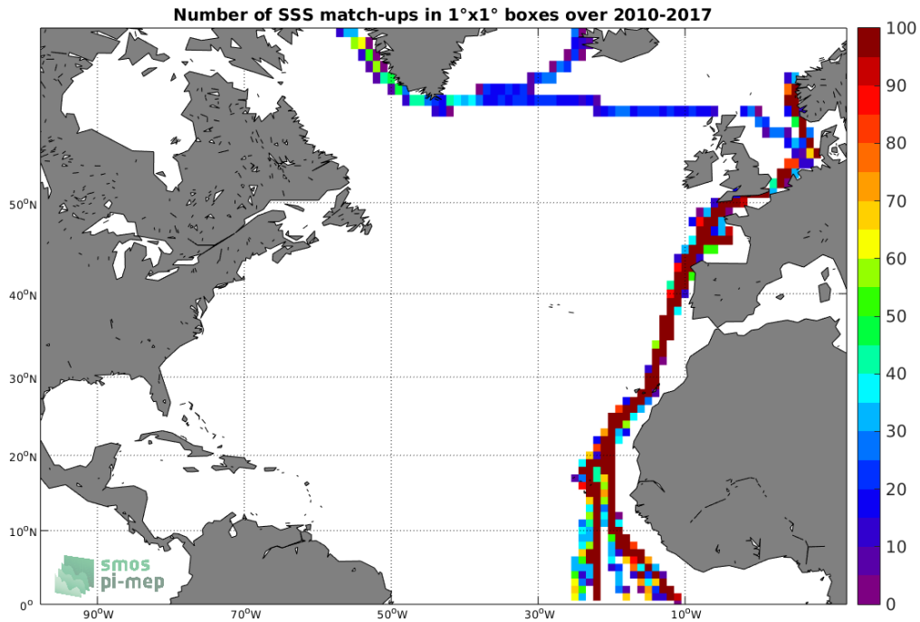
Figure 4: Number of SSS match-ups between TSG-POLARSTERN SSS and the SMOS-L3-CATDS-CECOS-LOCEAN-V3-18DAYS-25KM SSS product for the North Atlantic Ocean Pi-MEP region over 1^\circ \times 1^\circ boxes and for the full satellite product period.
