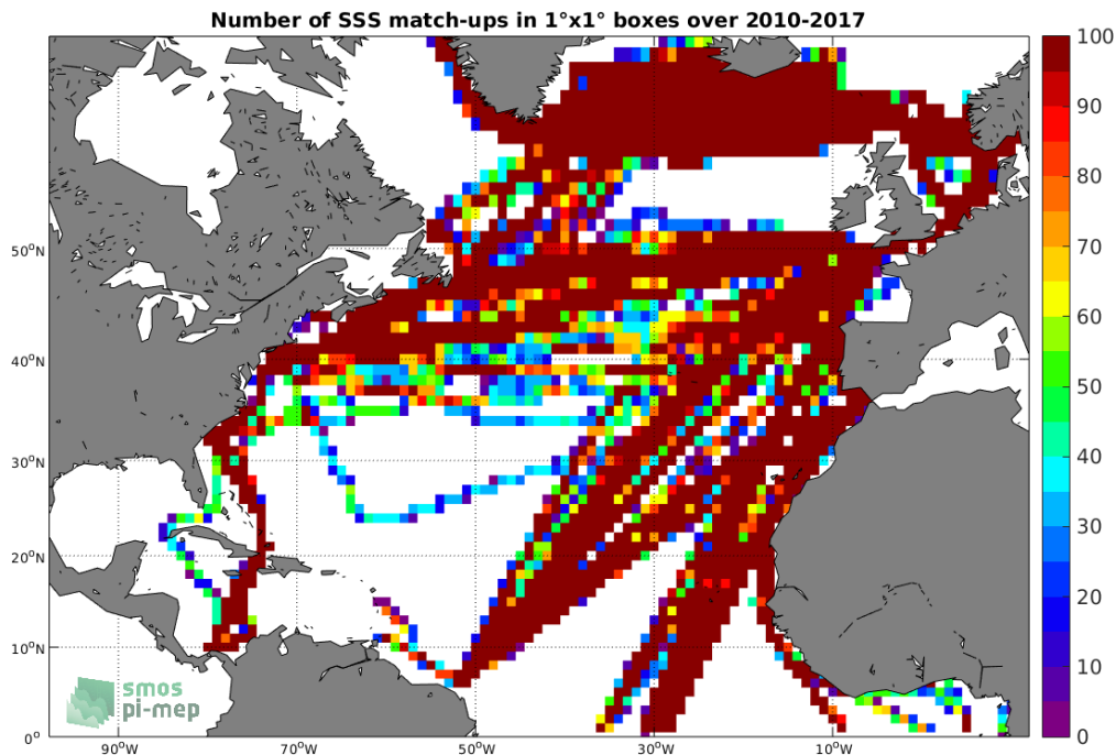
Figure 4: Number of SSS match-ups between TSG-LEGOS-DM SSS and the SMOS-L3-CATDS-CECOS-LOCEAN-V3-18DAYS-25KM SSS product for the North Atlantic Ocean Pi-MEP region over 1^\circ \times 1^\circ boxes and for the full satellite product period.
