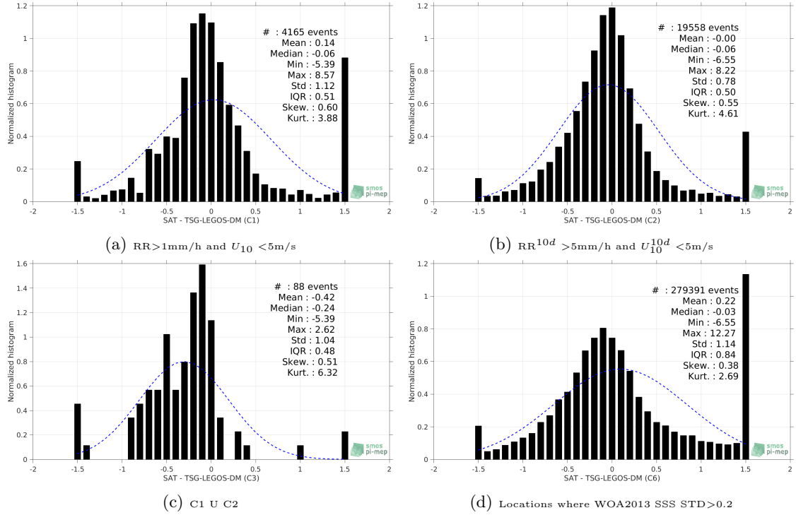
Figure 13: Normalized histogram of \Delta SSS (SMOS-L3-CATDS-CECOS-LOCEAN-V3-18DAYS-25KM - TSG-LEGOS-DM) for 6 different subdatasets corresponding to: RR > 1mm/h and U_{10} < 5 m/s (a), RR 10d > 5mm/h and U_{10}^{10d} < 5 m/s (b), C1 U C2 (c), Locations where WOA2013 SSS STD > 0.2 (d).
