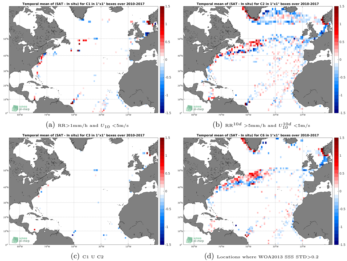
Figure 12: Temporal mean gridded over spatial boxes of size 1^\circ \times 1^\circ of \Delta SSS (SMOS-L3-CATDS-CECOS-LOCEAN-V3-18DAYS-25KM - TSG-LEGOS-DM) for 4 different subdatasets corresponding to: RR > 1\text{mm/h} and U_{10} < 5\text{m/s} (a), RR^{10d} > 5\text{mm/h} and U_{10}^{10d} < 5\text{m/s} (b), C1 U C2 (c), Locations where WOA2013 SSS STD > 0.2 (d).
