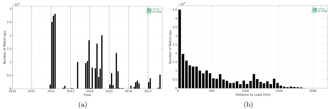
Figure 1: Number of match-ups between TSG-GOSUD-Sailing-ship and SMOS-L3-CATDS-CECOS-LOCEAN-V3-18DAYS-25KM SSS as a function of time (a) and as function of the distance to coast (b) over the North Atlantic Ocean Pi-MEP region and for the full satellite product period.
