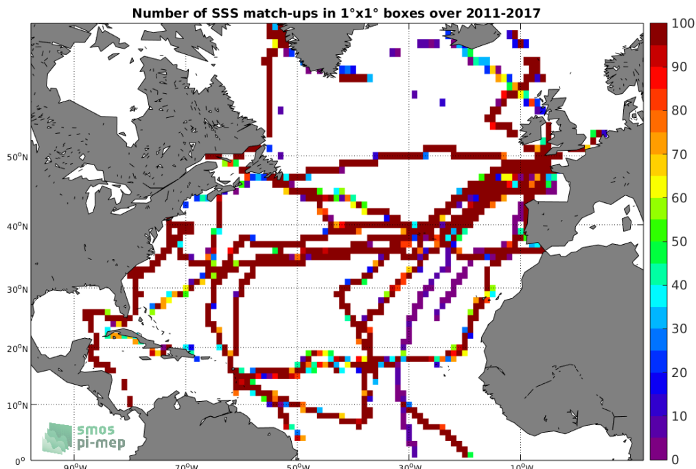
Figure 4: Number of SSS match-ups between TSG-GOSUD-Sailing-ship SSS and the SMOS-L3-CATDS-CECOS-LOCEAN-V3-18DAYS-25KM SSS product for the North Atlantic Ocean Pi-MEP region over 1^\circ \times 1^\circ boxes and for the full satellite product period.
