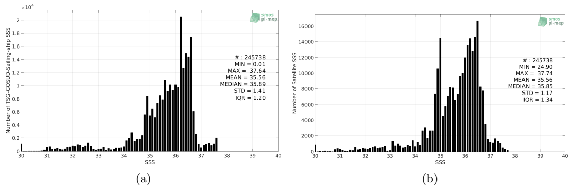
Figure 2: Histograms of SSS from TSG-GOSUD-Sailing-ship (a) and SMOS-L3-CATDS-CECOS-LOCEAN-V3-18DAYS-25KM (b) considering all match-up pairs per bins of 0.1 over the North Atlantic Ocean Pi-MEP region and for the full satellite product period.
