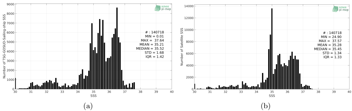
Figure 2: Histograms of SSS from TSG-GOSUD-Sailing-ship (a) and SMOS-L3-CATDS-CECOS-LOCEAN-V3-18DAYS-25KM (b) considering all match-up pairs per bins of 0.1 over the North Atlantic Ocean Pi-MEP region and for the full satellite product period.
